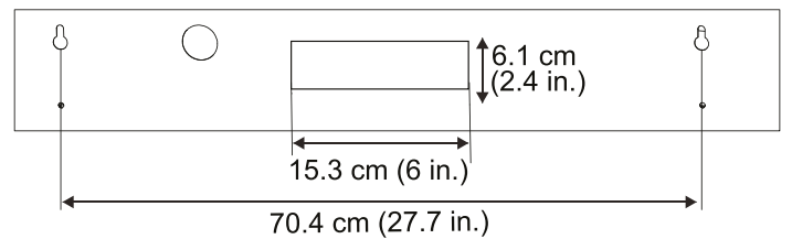
Rear view
