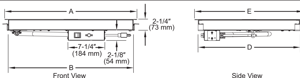
GRSBF Model Dimensions
