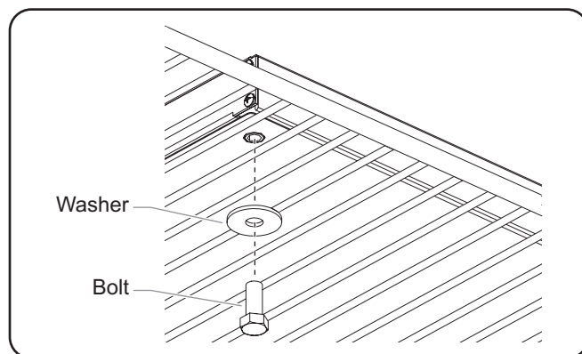
Wire Rack Mounting Kit Installation
