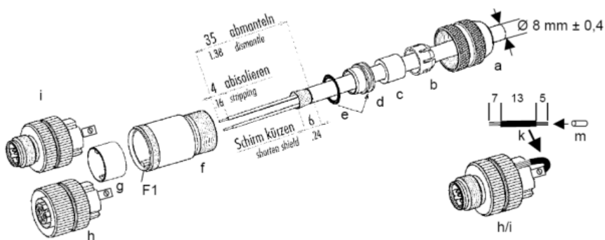
Figure 6-22 Inserting the bus cables in the M12 connector 6GK1 905-0Ex00
