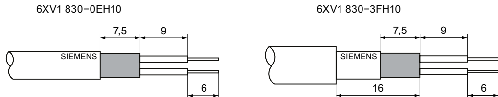
Figure 6-12 Length of cable stripped for connection to bus connector (6ES7 972-0B.12 ...)
