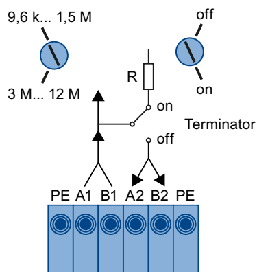
Figure 6-25 Control elements
