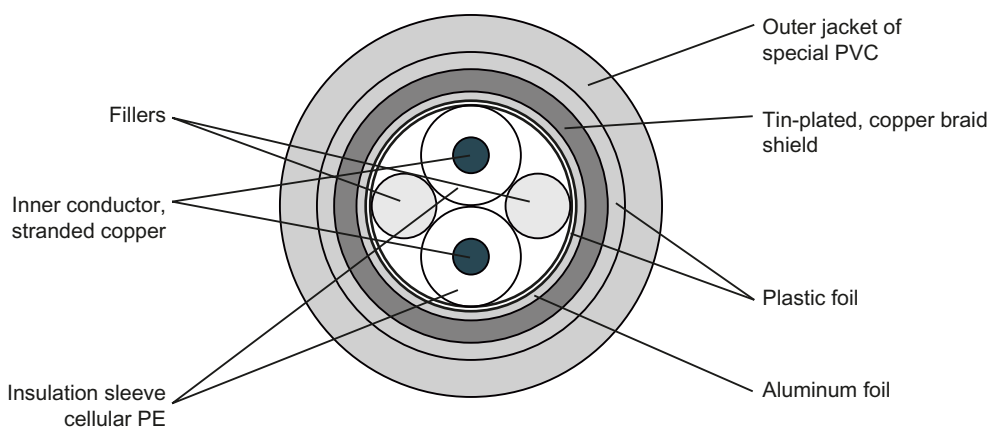
Figure 5-10 Structure of the festoon cable
