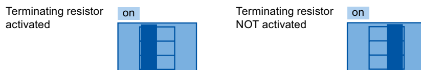
Figure 4-3 Setting of the terminating resistor
