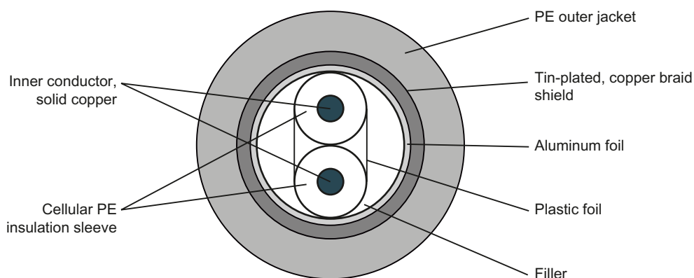
Figure 5-4 Structure of the bus cable with PE jacket
