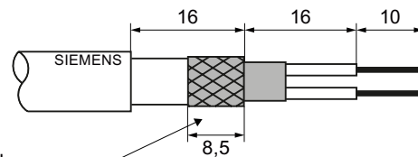
Figure 4-12 Stripping length for connecting to the PROFIBUS terminator
