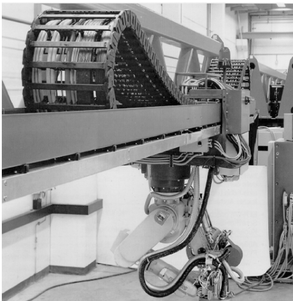
Figure 5-8 Example of using the PROFIBUS trailing cable in a drag chain
