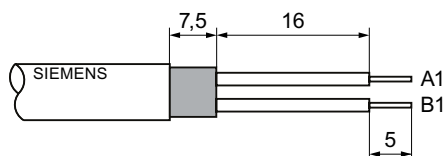
Figure 6-15 Length of cable stripped for connection to bus connector (6ES7 972-0Bx41...)
