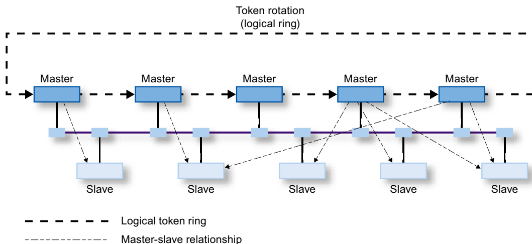
Figure 1-2 Principle of the PROFIBUS medium access technique
