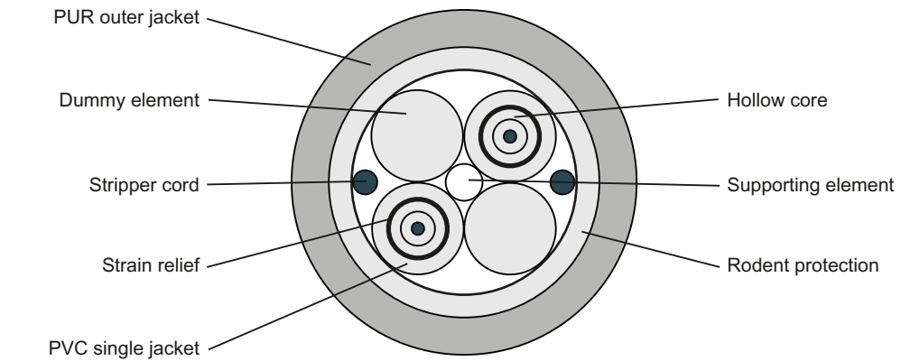
Figure 7-13 Design of the fiber-optic trailing cable
