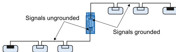
Figure 4-9 Ungrounded operation of bus segments
