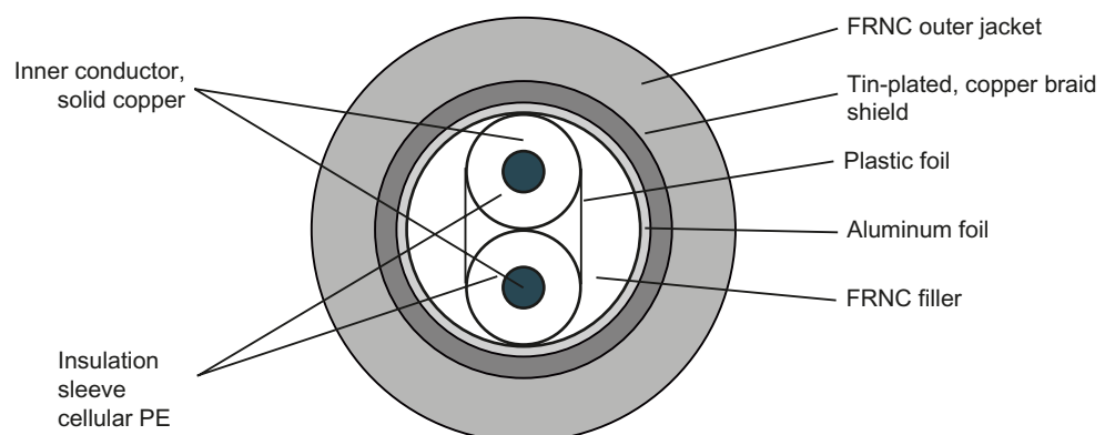
Figure 5-3 Structure of the bus cable with halogenfree outer jacket
