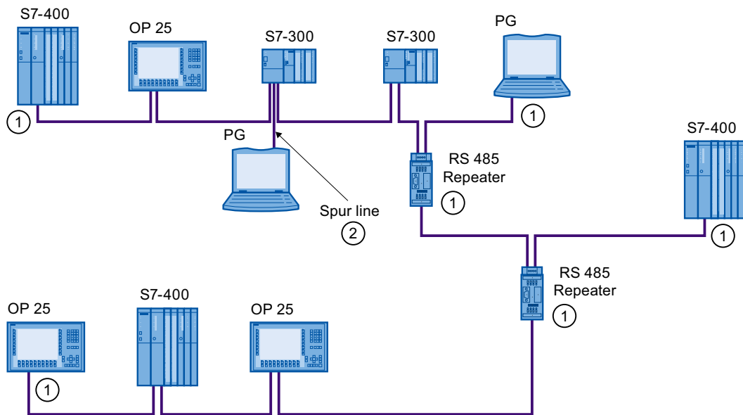
Figure 2-1 Topology with RS-485 technology
