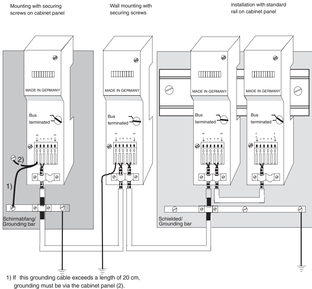
Figure 6-28 Ways of installing and grounding the bus terminal
