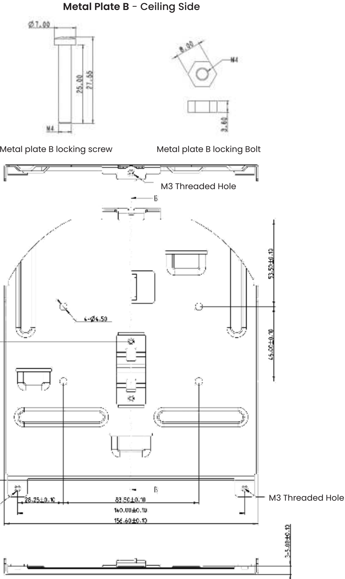
Metal Plate B - Ceiling Side
