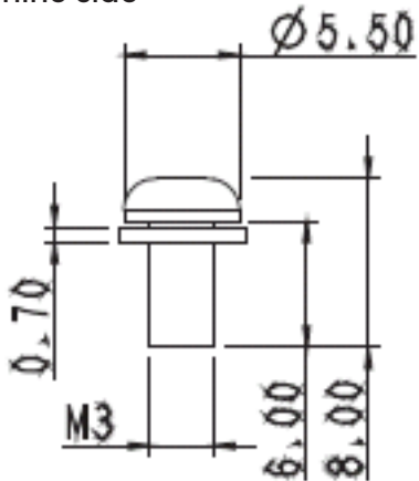
Metal plate A - Locking Screw
