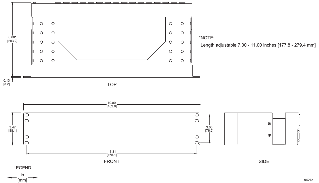
Figure 13 Adjustable Rack-Mount Adapter Panel
