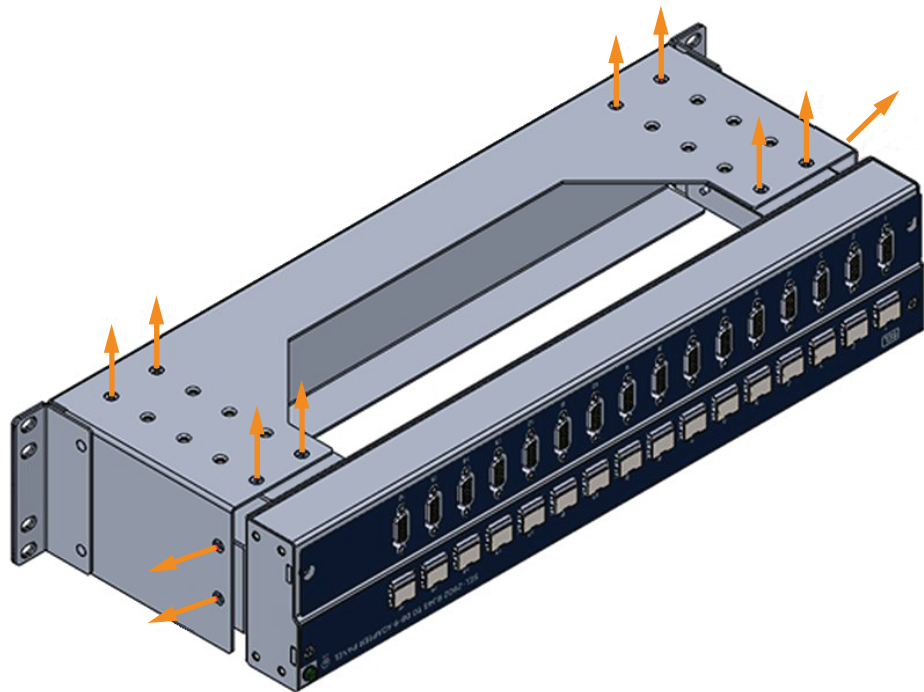
Figure 7 Remove Screws
