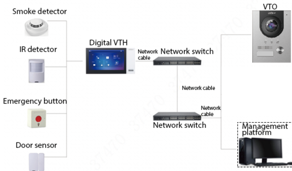
Figure 1-1 Network diagram
