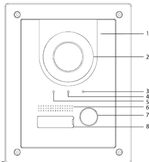
Figure 2-4 Front panel
