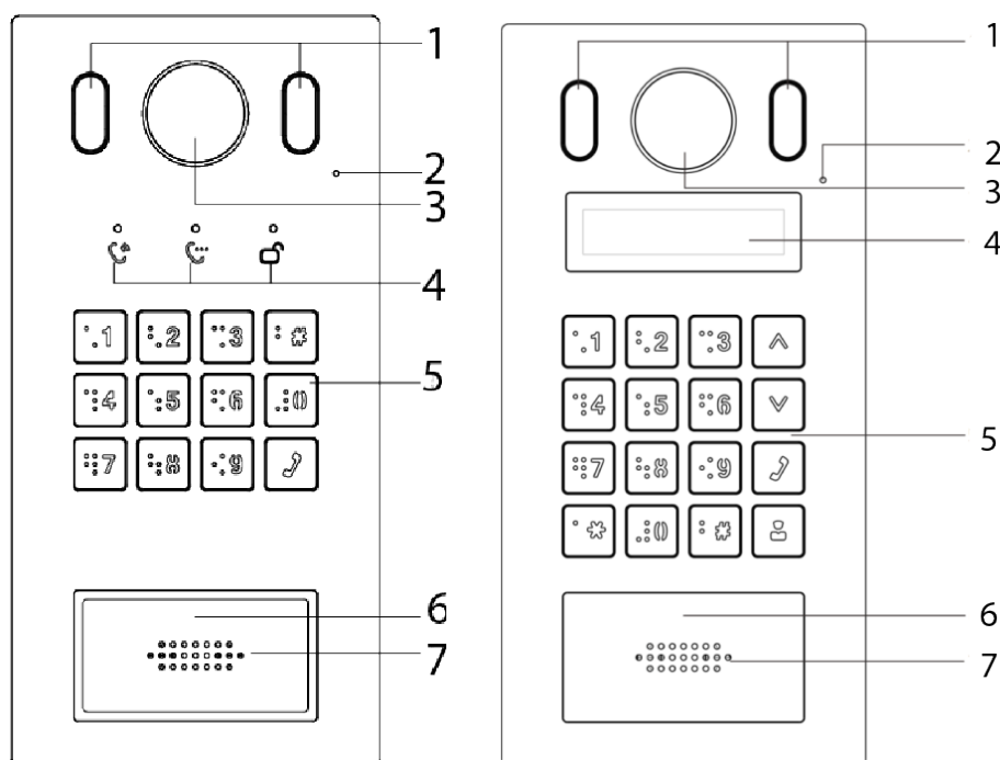
Figure 2-12 Front panel
