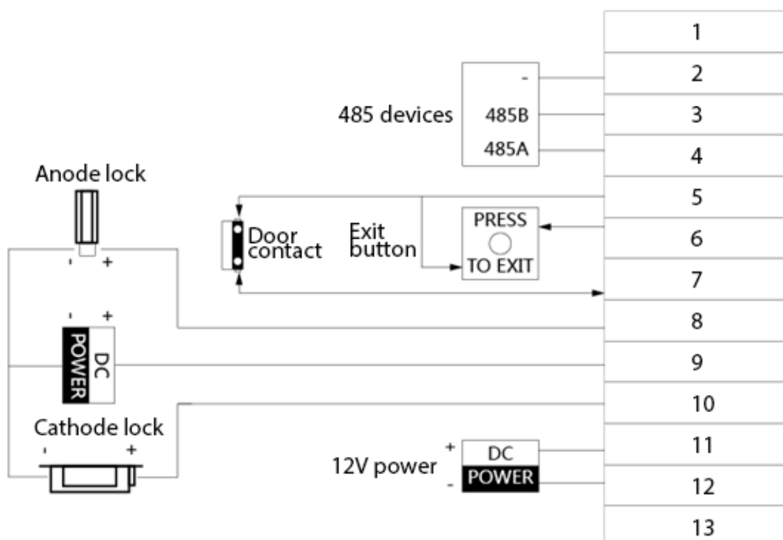
Figure 2-8 Cable connection
