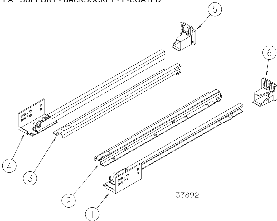
133892 CONCEALED RUNNER DRAWERS
