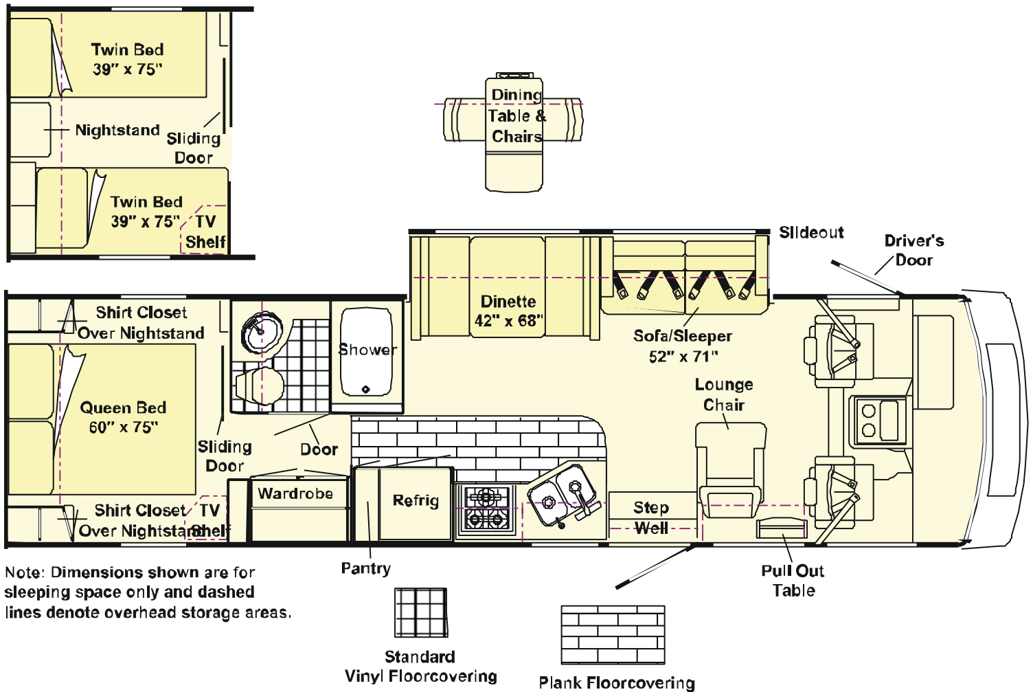
FLOORPLAN
