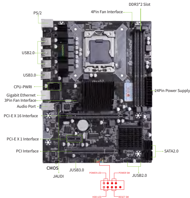
1-1 X58-RX 3.0 Motherboard illustration
