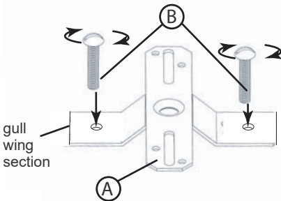
Drawin g 1 – Mounting strap preperation
