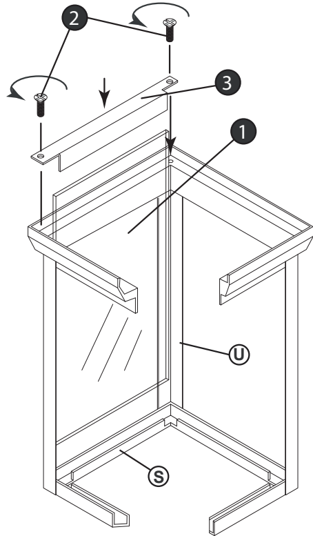
DRAWING 1 - Scroll install
