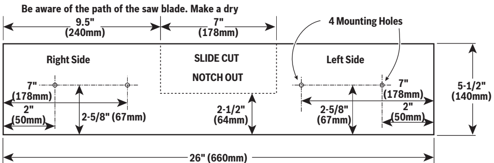
Fig. 39 Tall Auxiliary Wood Fence - 3/4" (19mm) Thick
