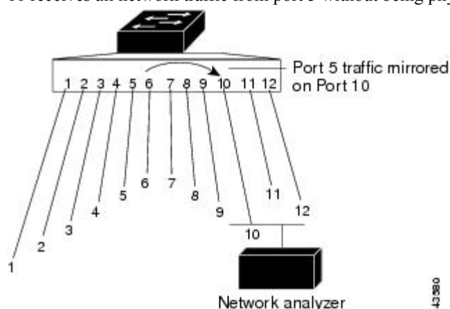
Figure 7: Example of Local SPAN Configuration on a Device Stack
