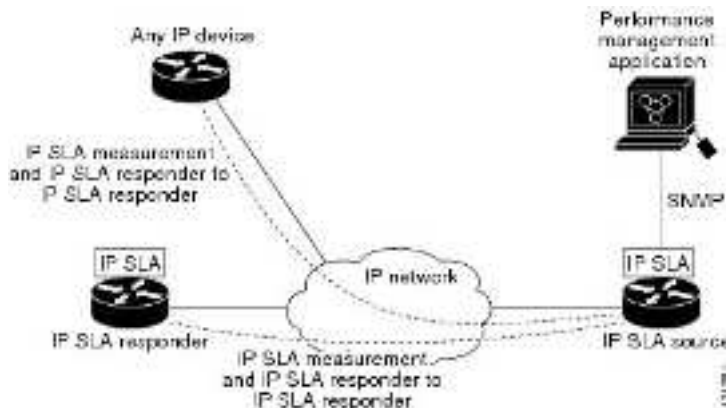
Figure 4: Cisco IOS IP SLAs Operation
