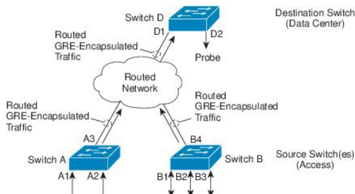
Figure 9: ERSPAN Configuration
