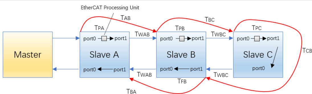
Figure 4. Propagation delay of each slave
