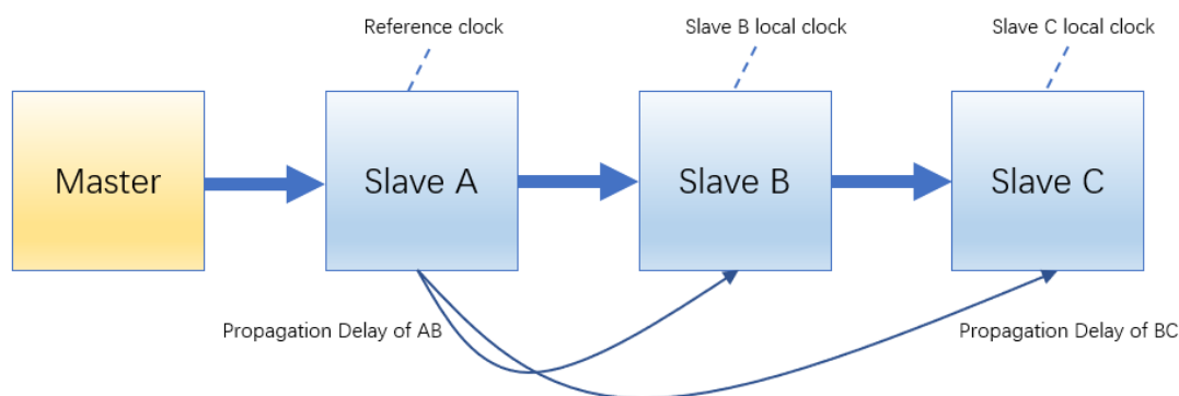
Figure 3. Distribute clock and propagation delay
