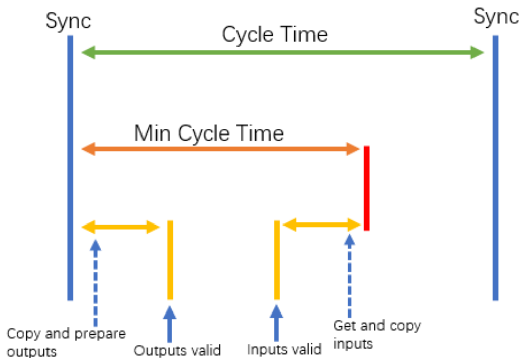
Figure 7. Normal DC mode
