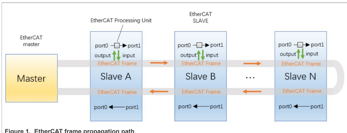
Figure 1. EtherCAT frame propagation path
