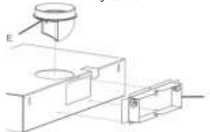
E. Round transition kit W11035218 F. Rectangular transition kit W11035219
