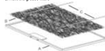
A. Anti-grease filter B. Charcoal filter C. Attachment rods
