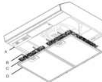
A. Hood assembly B. Charcoal filter attachment rod C. Charcoal filter 31.5" (80 cm) model - W11035220 30" (76 cm) model - W11035759 23.6" (60 cm) model - W11035760 D. Anti-grease filter
