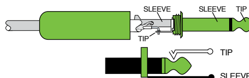
Unbalanced 1/4" Connectors
