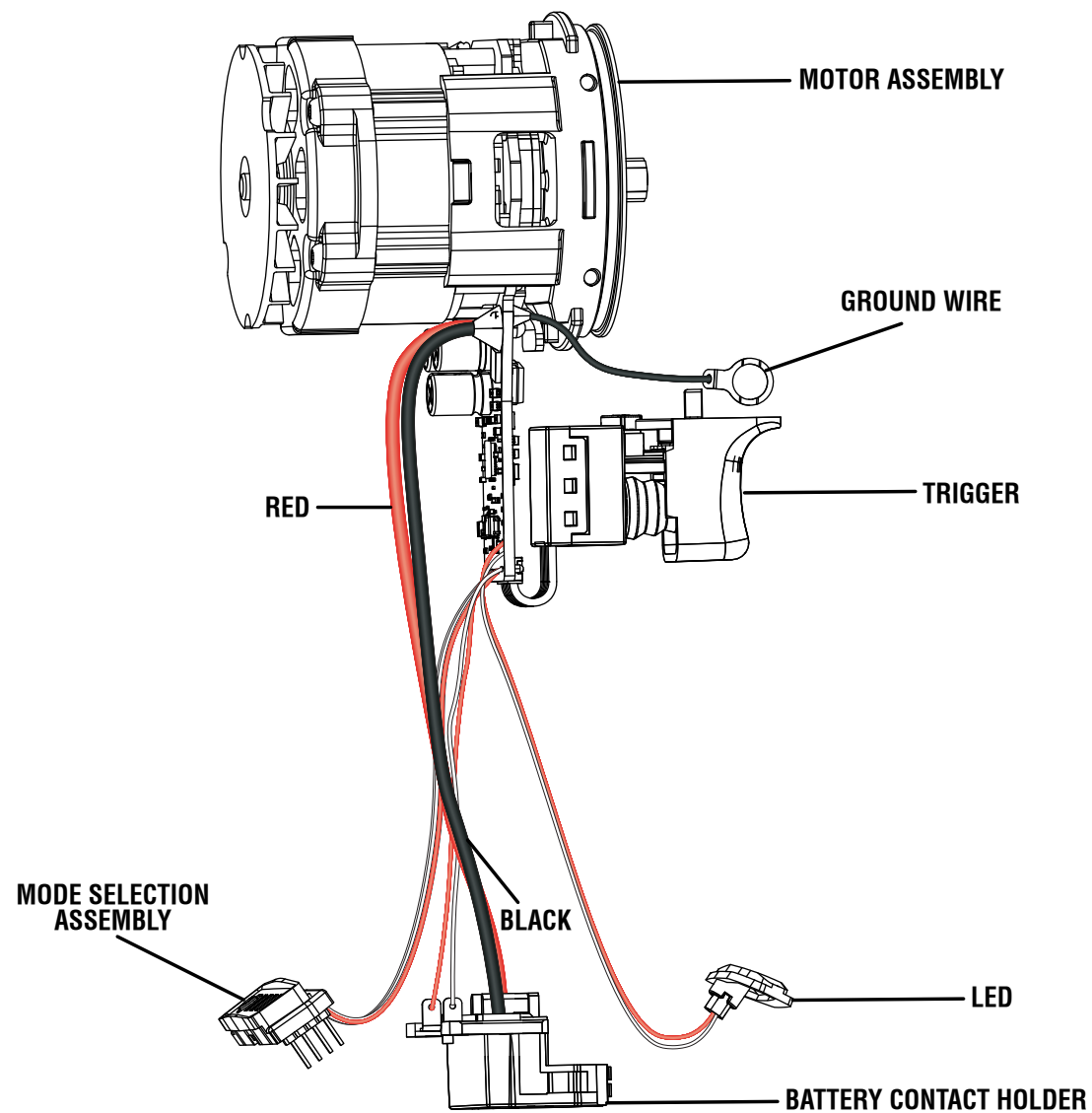
WIRING DIAGRAM
