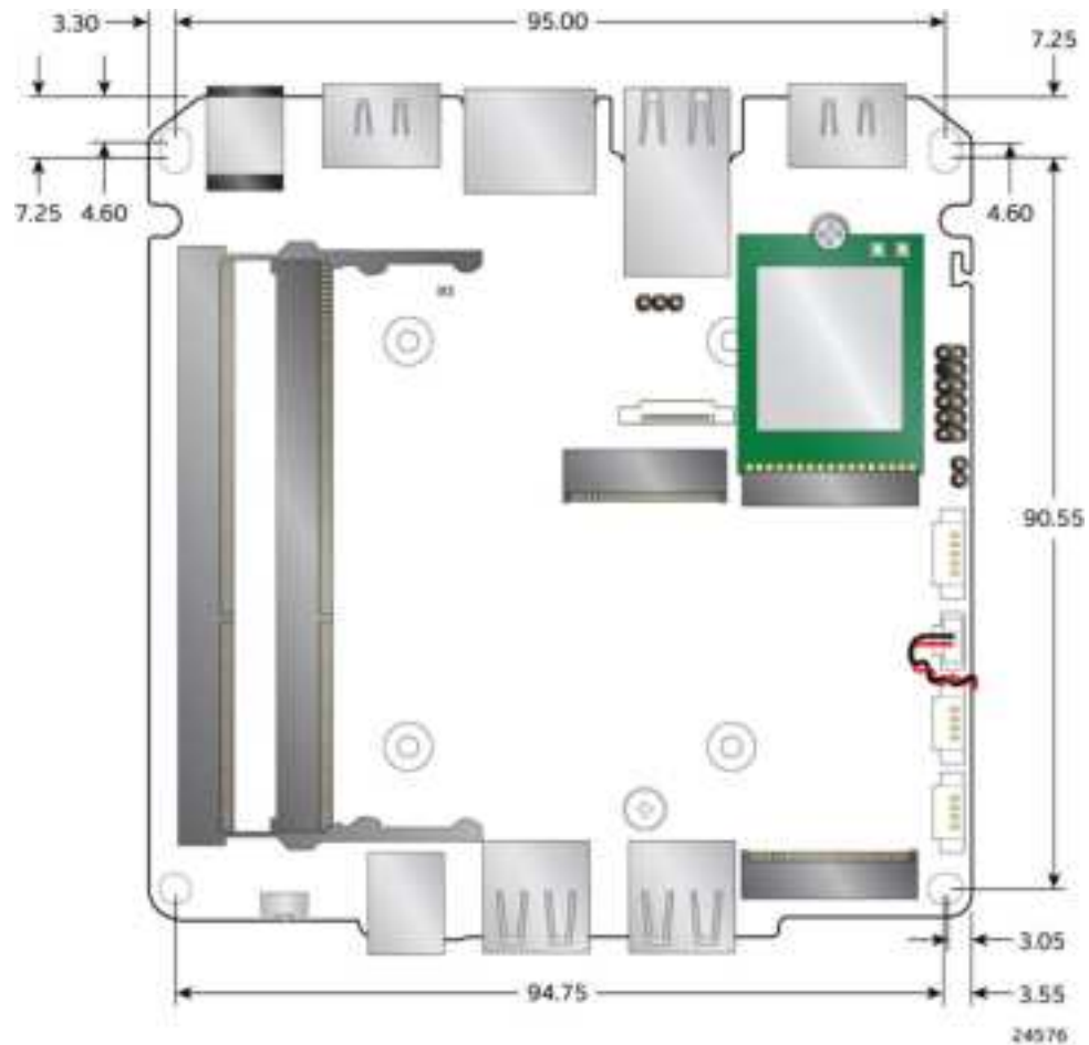
Figure 15. Board Dimensions
