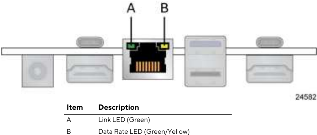
Figure 7. LAN Connector LED Locations
