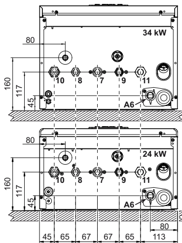
fig. 35- Bottom view
