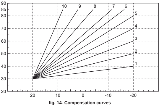
fig. 14- Compensation curves
