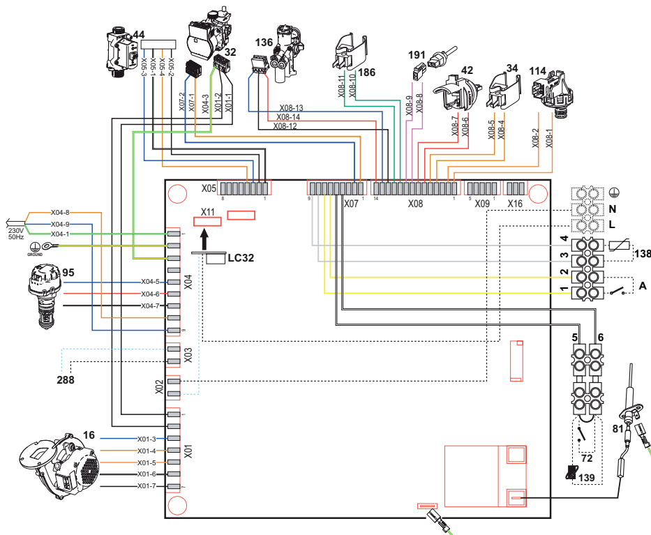
fig. 40- Wiring diagram
