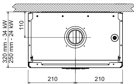
fig. 34- Top view
