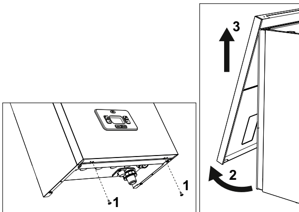
fig. 30- Front panel opening
