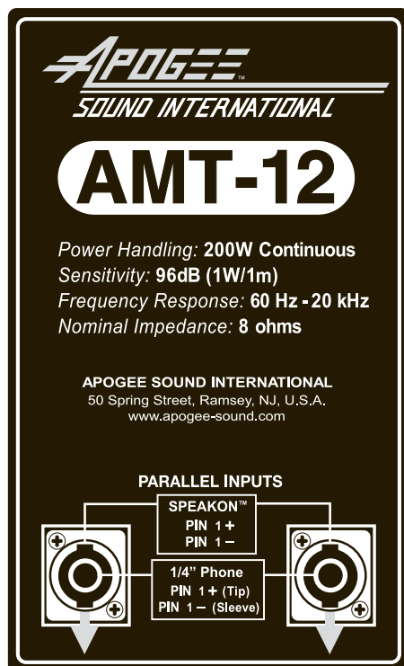
AMT-12 Panel
