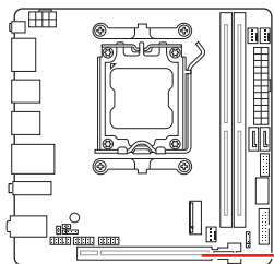
PCI_E1: PCIe 5.0 x16 (From CPU)
