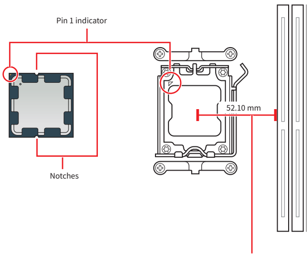
Distance from the center of the CPU socket to the nearest DIMM slot.
