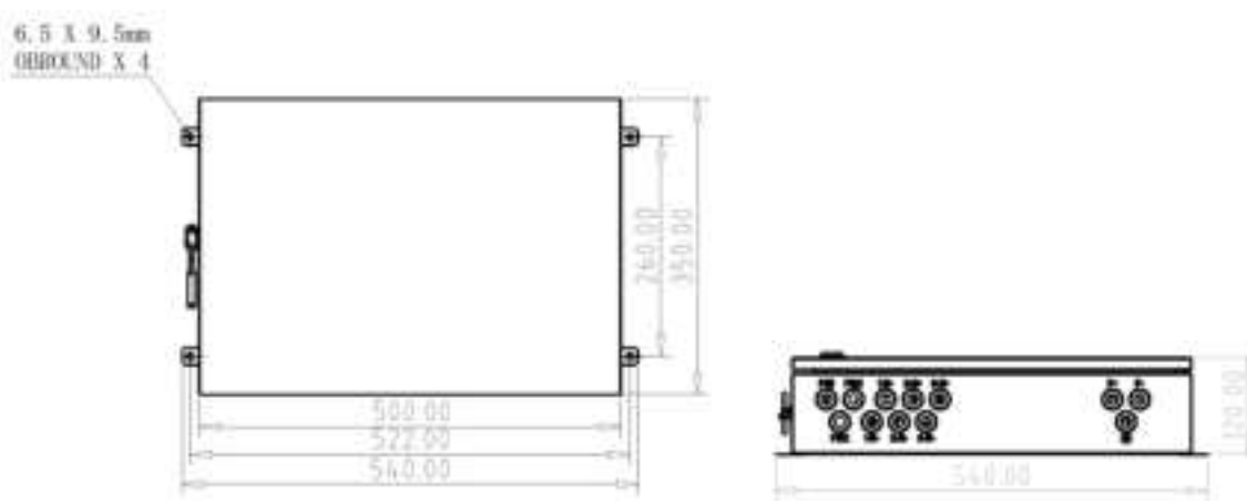
Figure 3 Dimensions of the Combiner Box
