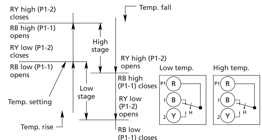
Figure 8 – Operational Sequence of Two-stage SPDT/SPDT Thermostats
