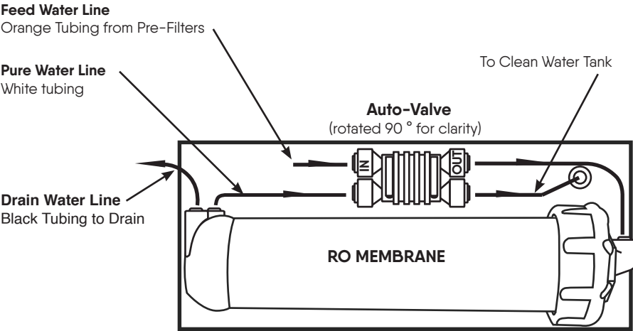
Figure 2 RO SYSTEM TOP VIEW
