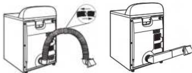
Periscope installation
