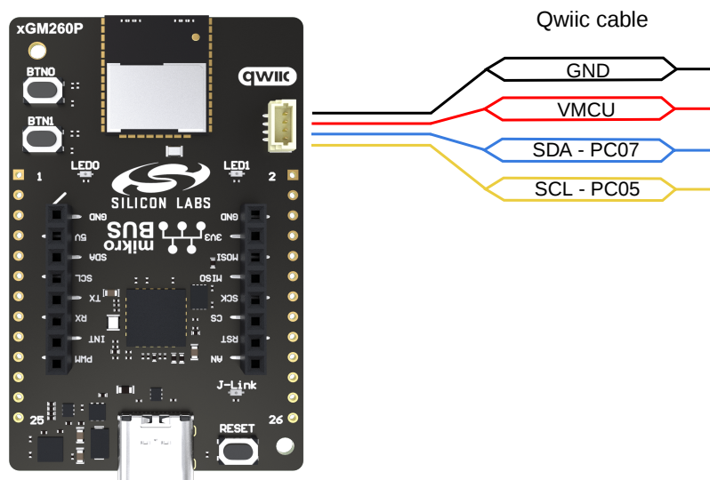
Figure 3.7. Qwiic Connector
