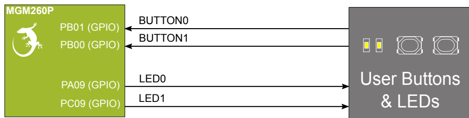
Figure 3.3. Buttons and LEDs
