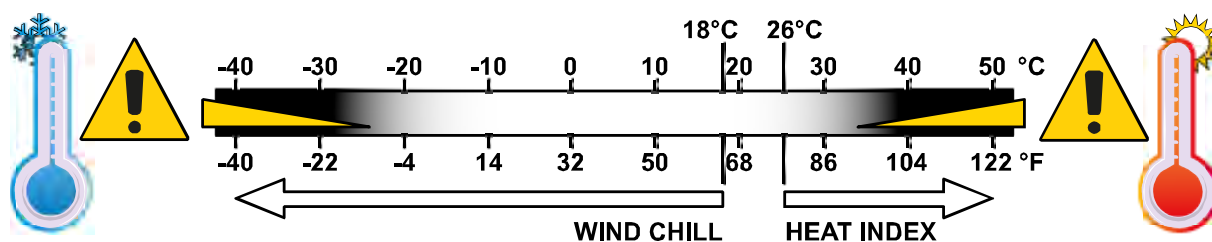
Illustration 5: Proportionality of heat index and wind chill.
