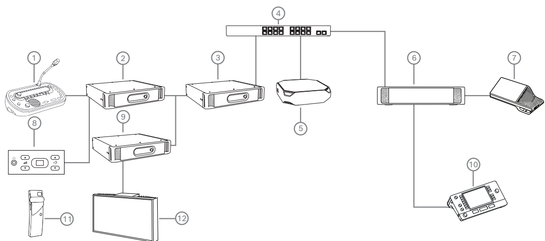
Figure 5.8: Interfacing DICENTIS with DCN NG
