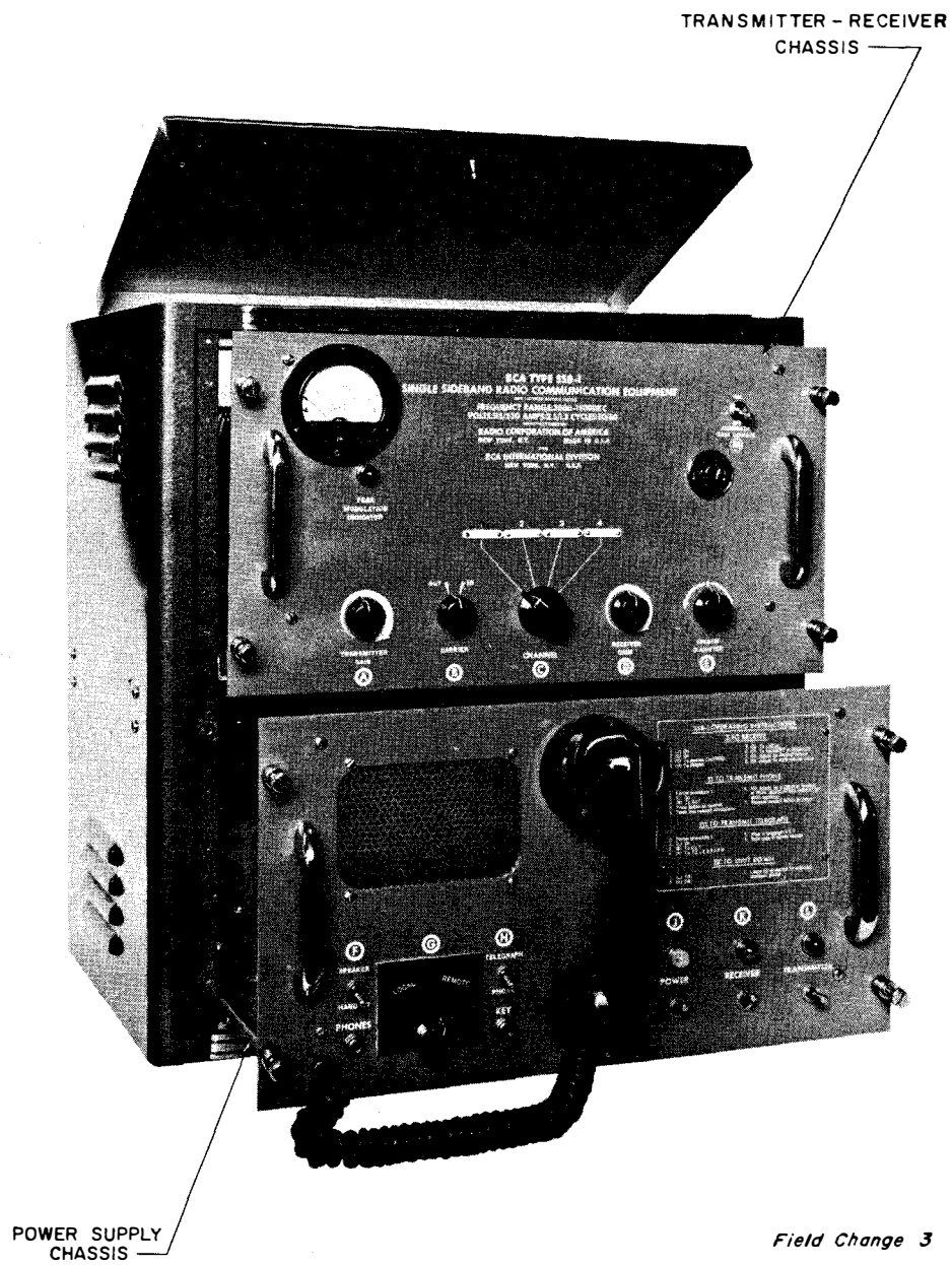
Figure 3. Cabinet Top Raised and Chassis Withdrawn
