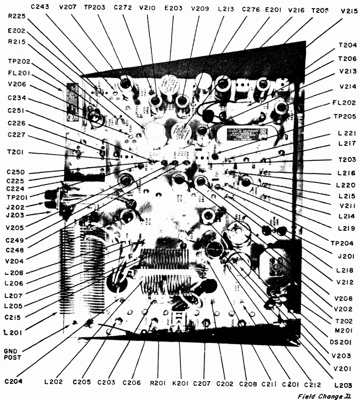
Figure 20. Transmitter-Receiver, Top View
