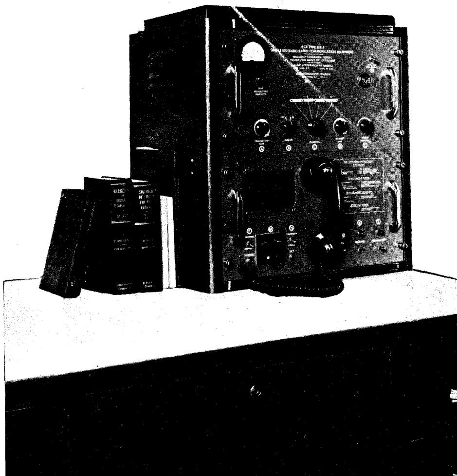
Figure 1. Desk Installation
