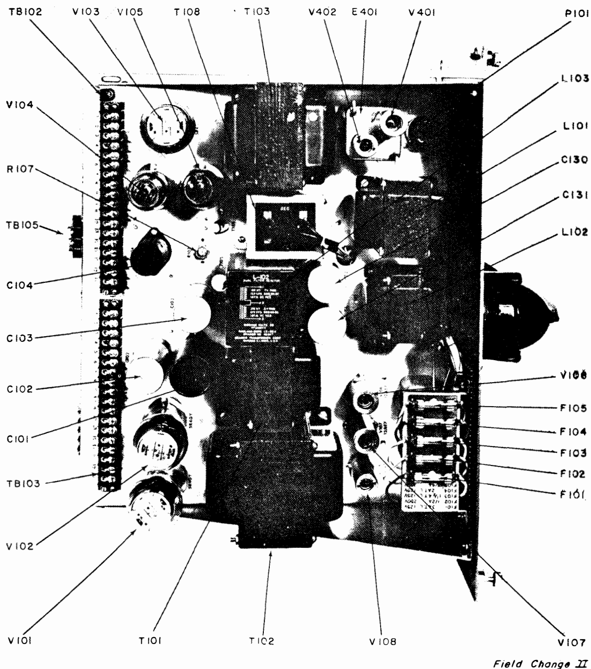
Figure 16. Power Supply, Top View
