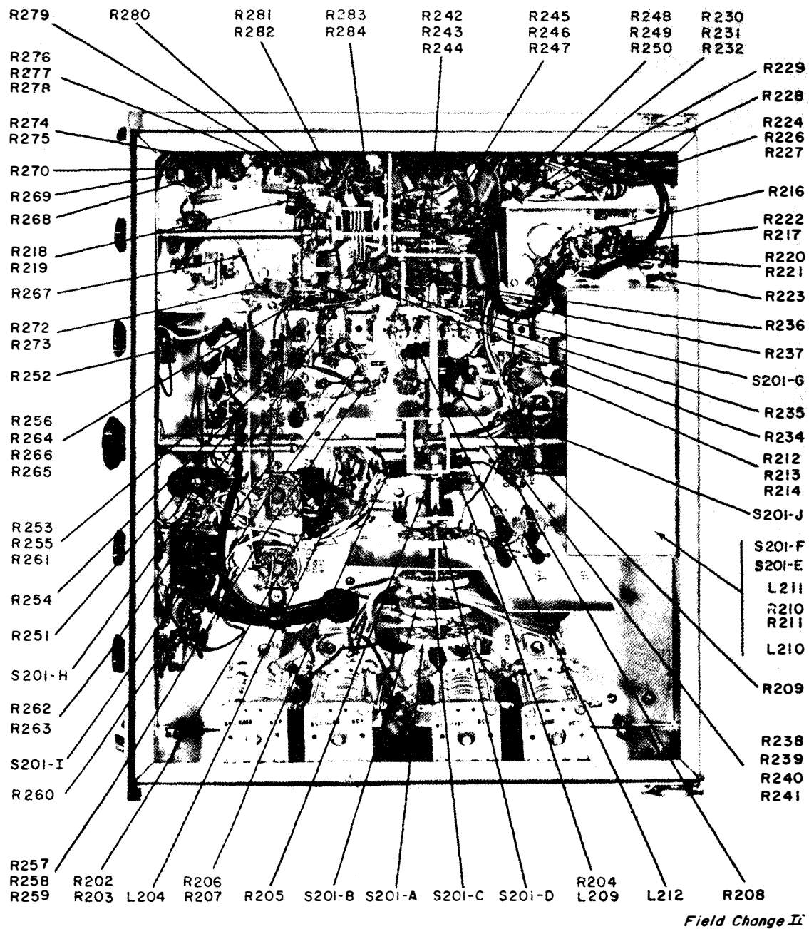
Figure 21B. Transmitter-Receiver, Bottom View, Location of Components other than Capacitors
