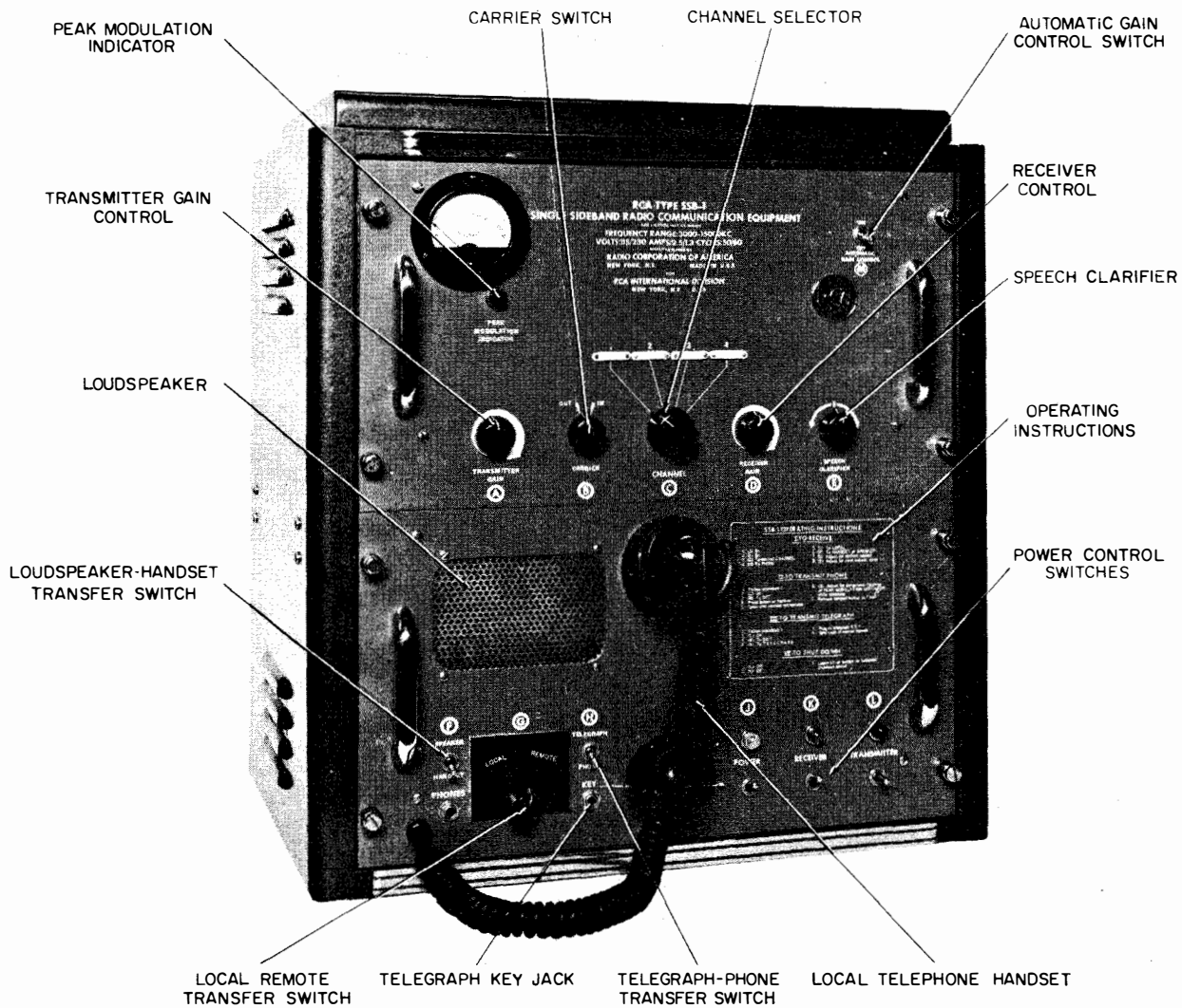
Figure 10. Front Panel Controls
