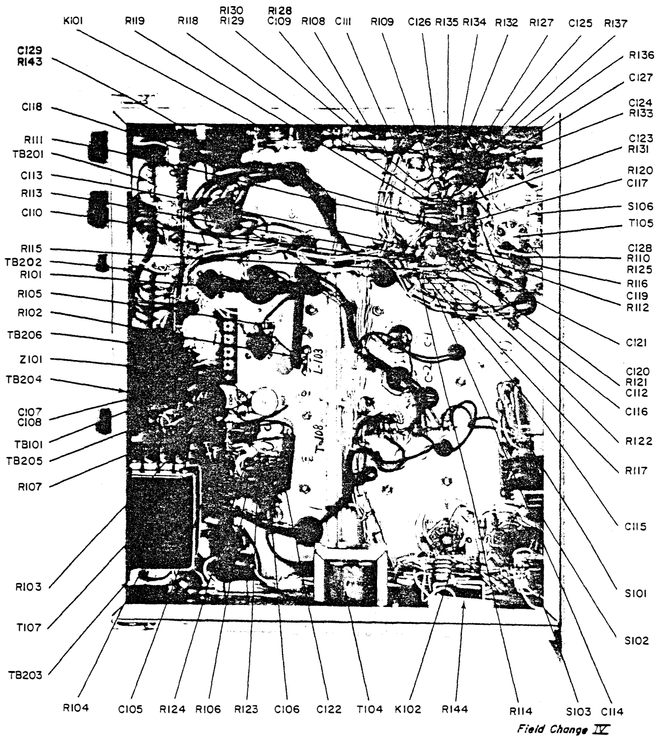
Figure 17. Power Supply, Bottom View
