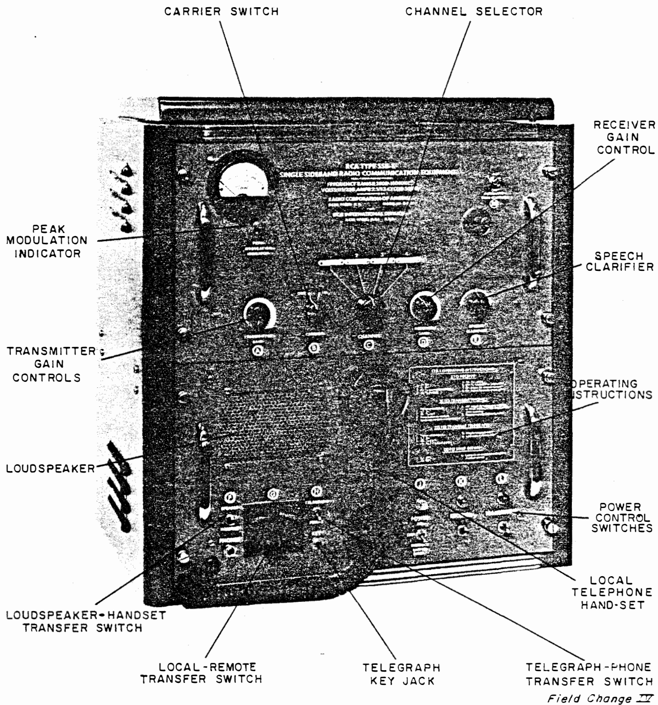
Figure 10. Front Panel Controls
