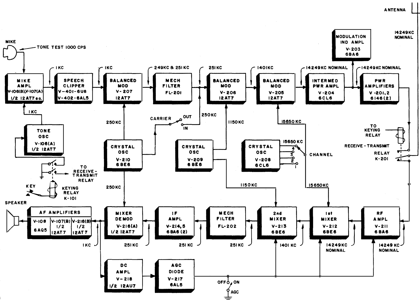
Figure 5. Block Diagram
