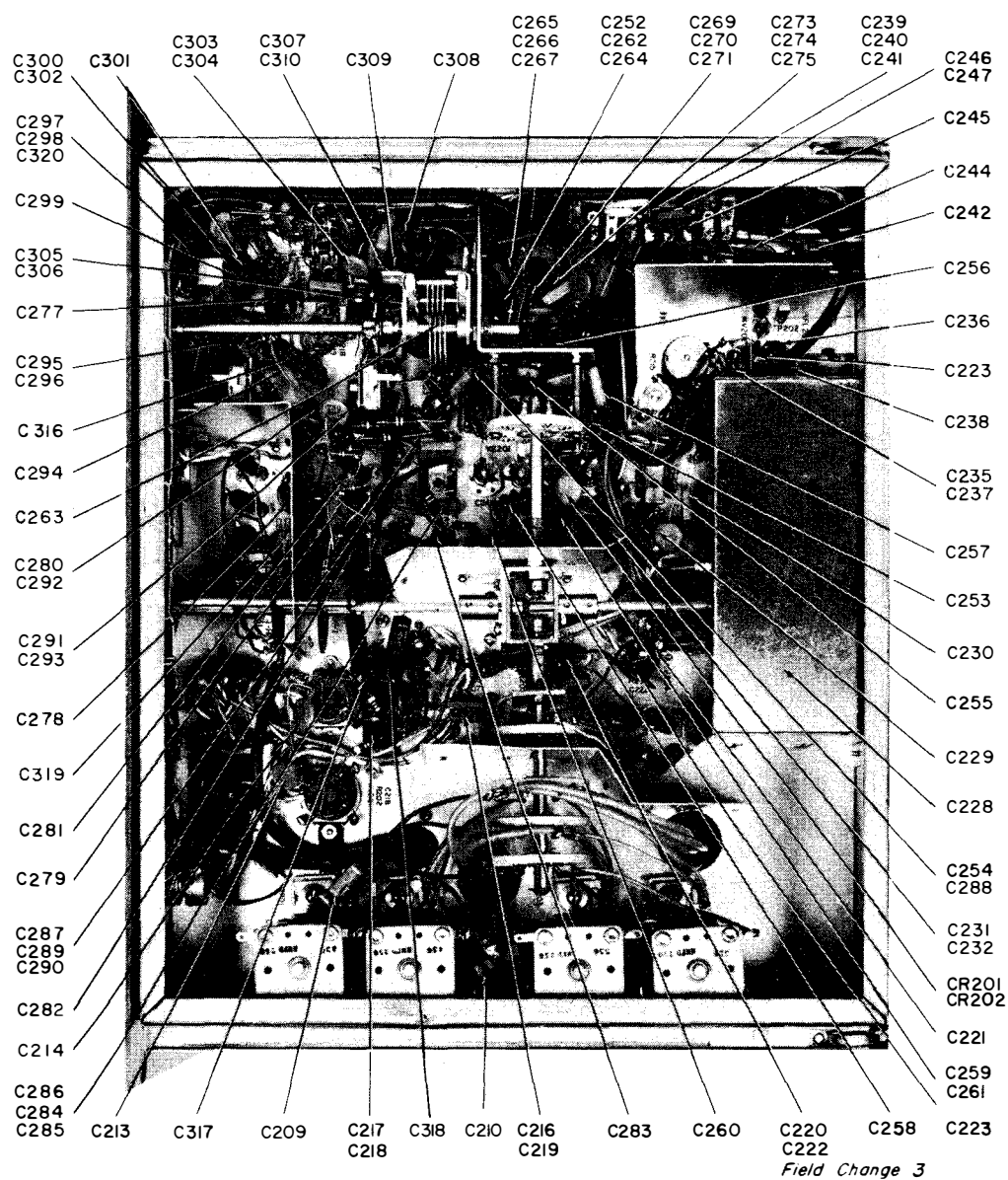
Figure 21A. Transmitter-Receiver, Bottom View, Location of Capacitors
