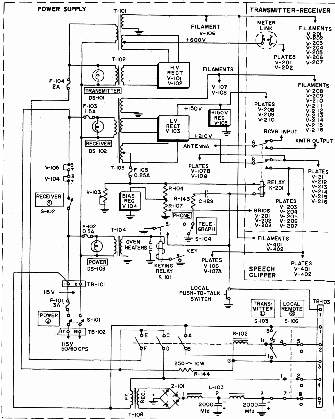
Figure 6. Power and Control Circuits
