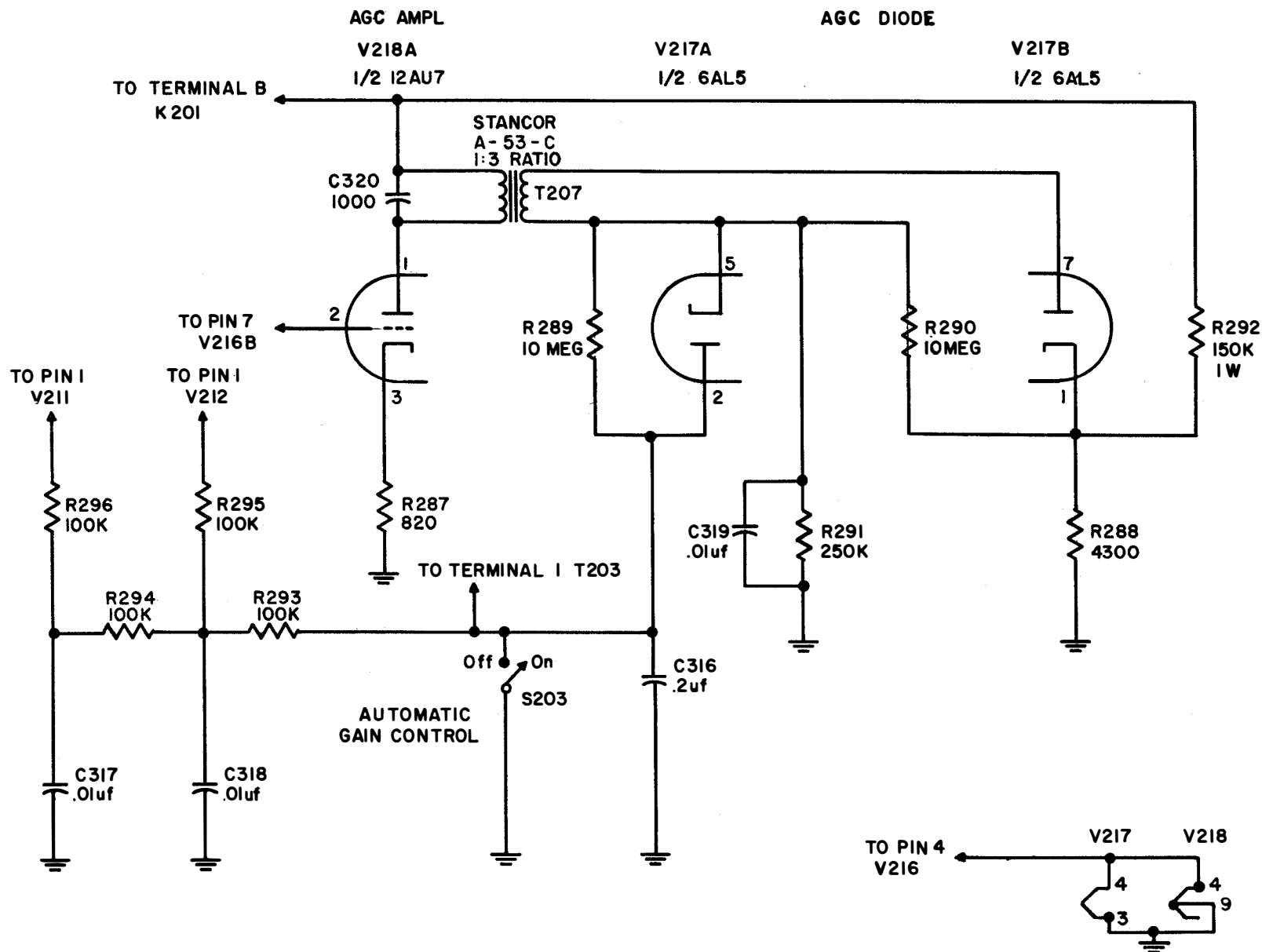
MODIFICATION TO TRANSMITTER RECEIVER SCHEMATIC
