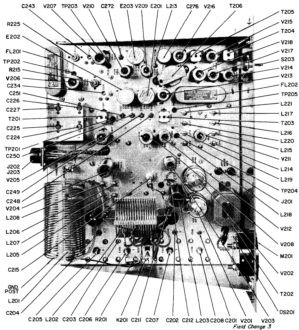
Figure 20. Transmitter-Receiver, Top View
