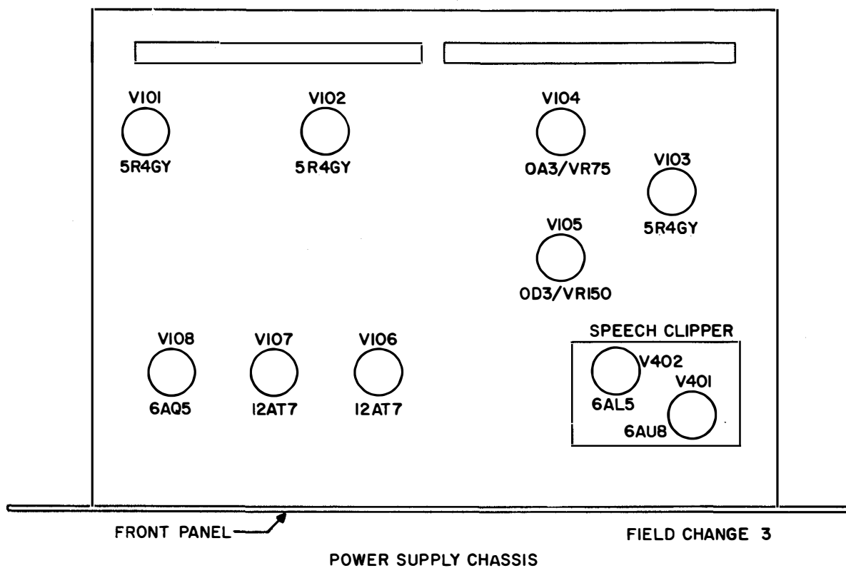
Figure 15. Tube Location Diagram
