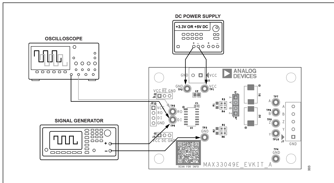
Figure 2. Connection Diagram
