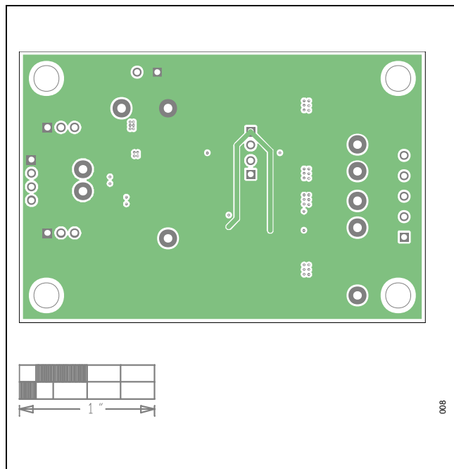
MAX33049E EV Kit PCB Layout—Layer 3 (VCC Layer)
