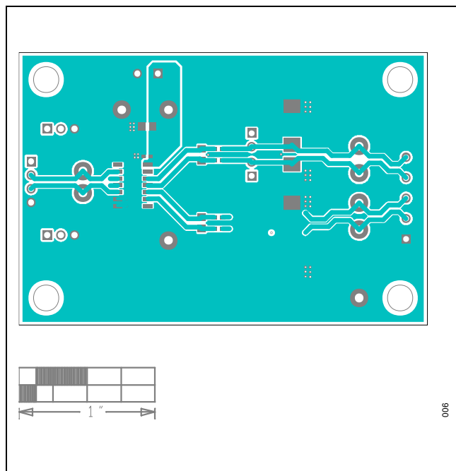
MAX33049E EV Kit PCB Layout—Top Layer
