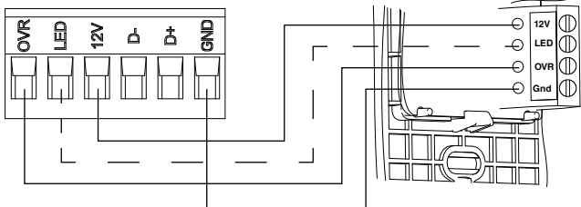
Remote 10 positions terminal
