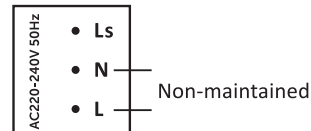
(Non-maintained operation)
