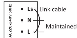
(Maintained operation)
