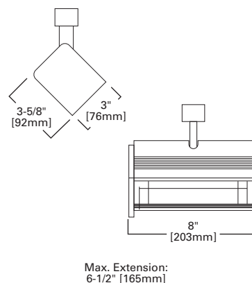
L1753 QUARTZ WALL WASHER
