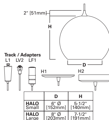
SMALL HALOID, LARGE HALOID
