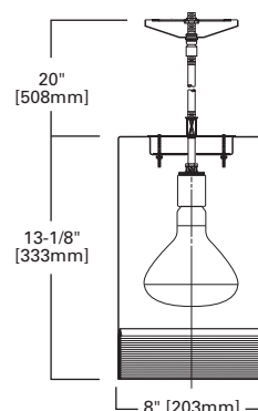
H1319 PENDANT MOUNT DOWNLIGHT
