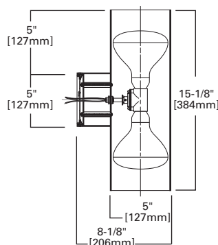
H2353 WALL MOUNT UPLIGHT/ DOWNLIGHT
