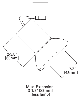
L4009 UNIVERSAL LAMPHOLDER
