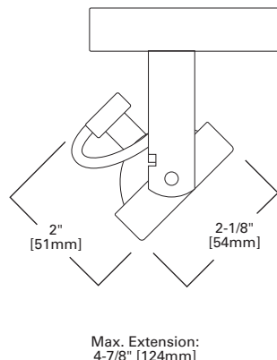
L2717 LV GIMBAL RING WITH INTEGRAL 12V TRANSFORMER
