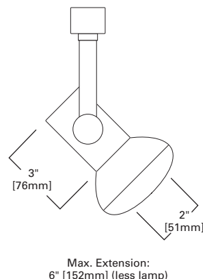
L702 UNIVERSAL LAMPHOLDER
