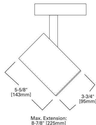
L2771 FLATBACK CYLINDER WITH BLACK BAFFLE
