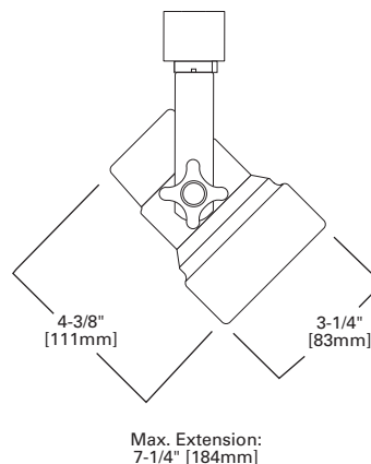
L1820 PAR20 STUDIO
