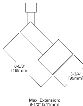
L732 CONTINENTAL CYLINDER WITH BAFFLE
