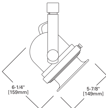
L1511 CLASSIC
