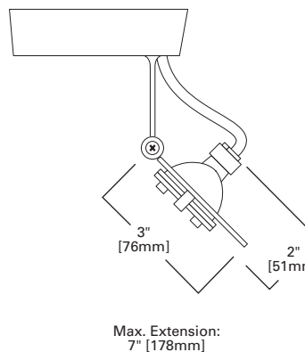
LZR404 LV PENDANT WITH TRANSFORMER
