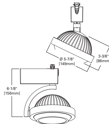
L806HO LED
