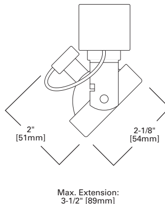
L2716 LOW VOLTAGE GIMBAL RING
