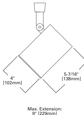
LZR307 FLATBACK CYLINDER WITH BAFFLE
