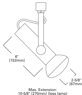
L700 UNIVERSAL LAMPHOLDER
