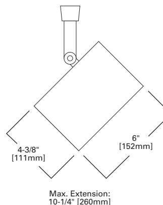
LZR308 FLATBACK CYLINDER WITH BAFFLE
