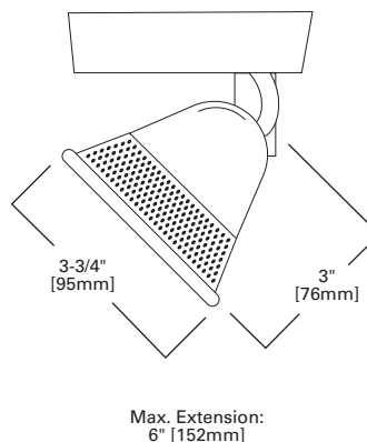
LZR402 LV PERFORATED BELL WITH TRANSFORMER
