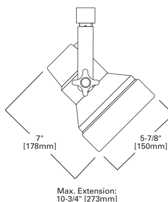
L1838 PAR38 STUDIO
