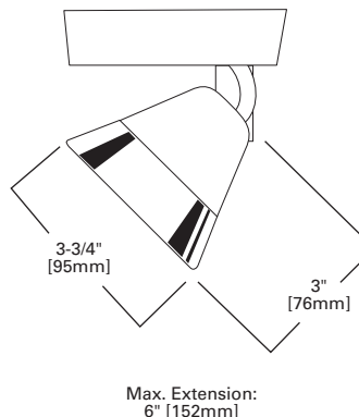
LZR403 LV GLASS BELL WITH TRANSFORMER
