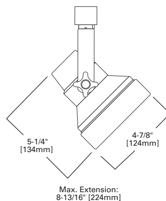
L1830 PAR30 STUDIO
