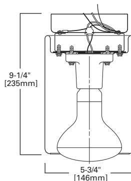
H2335 R40 OPEN DOWNLIGHT
