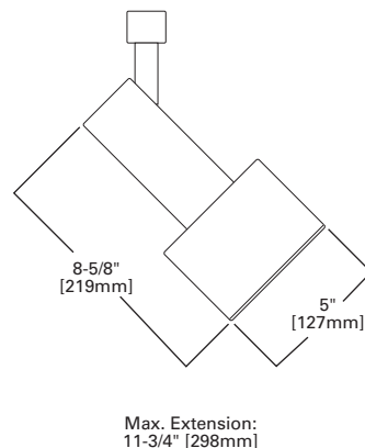
L733 CONTINENTAL CYLINDER WITH BAFFLE
