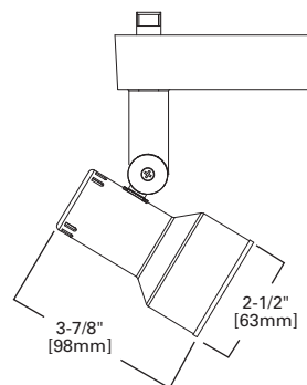
LZR406 LV STEP CYLINDER WITH TRANSFORMER
