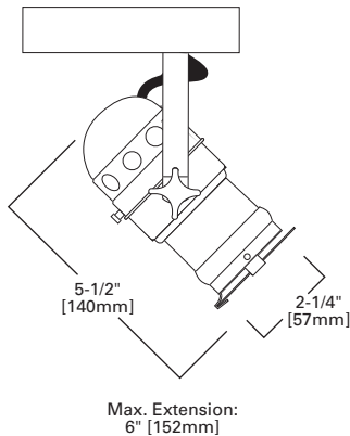
L1816 LOW VOLTAGE STUDIO CLASSIC
