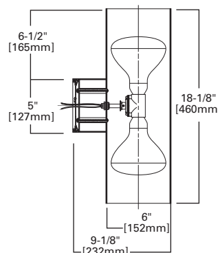
H2355 WALL MOUNT UPLIGHT/ DOWNLIGHT OPEN
