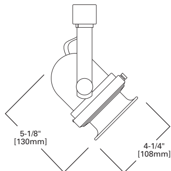
L1510 CLASSIC
