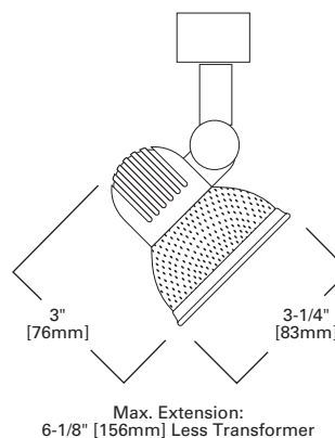
L2701 LOW VOLTAGE FIXTURE WITH PERFORATED SHADE
