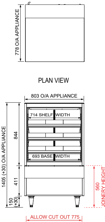
FRONT ELEVATION
