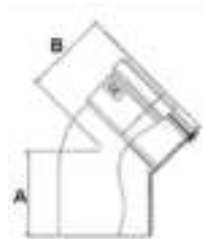
EF80 A=72.5mm, B=72.5mm
