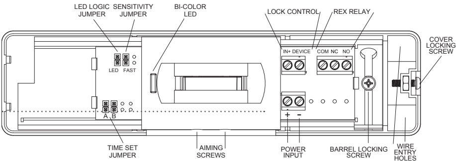
Diagram 9 XMS2 Overview
