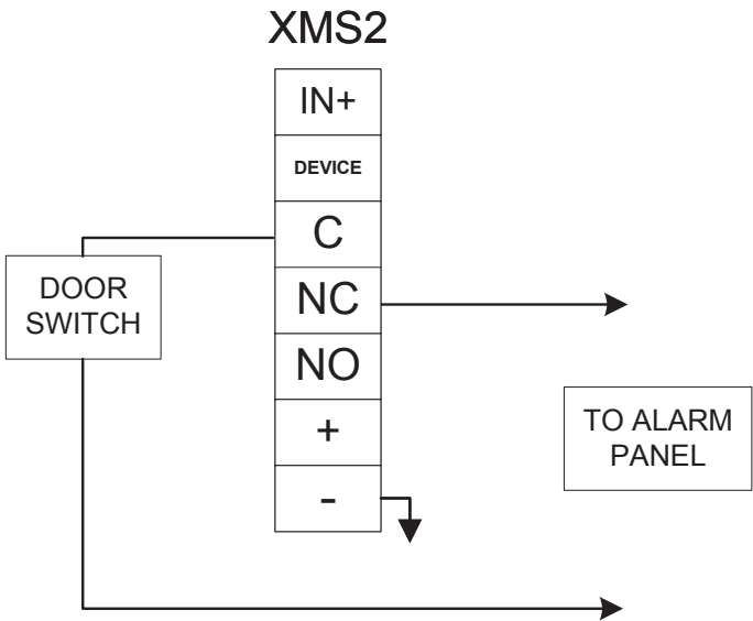
Diagram 13 Alarm Signal Open with Door Closed
