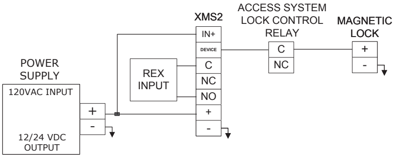
Diagram 14 Wiring with an Access Control System
