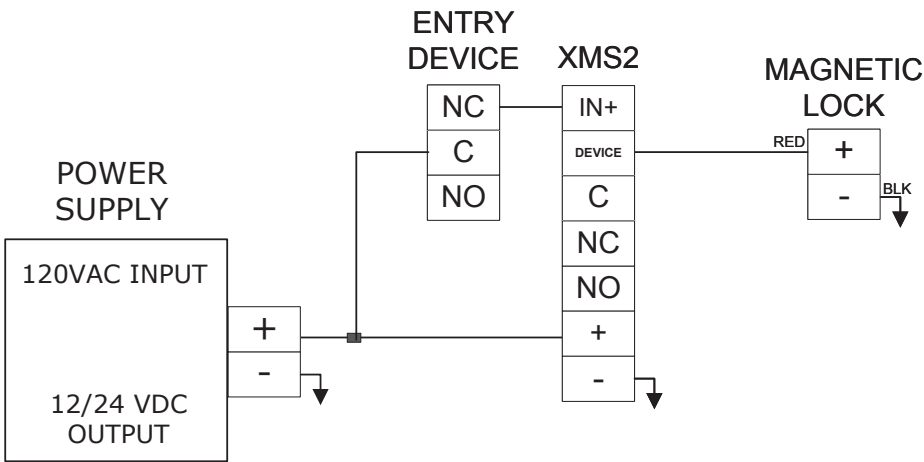
Diagram 11 Wiring with Entry Device
