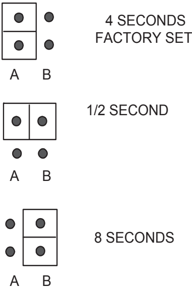
Diagram 16 Time Set Jumper
