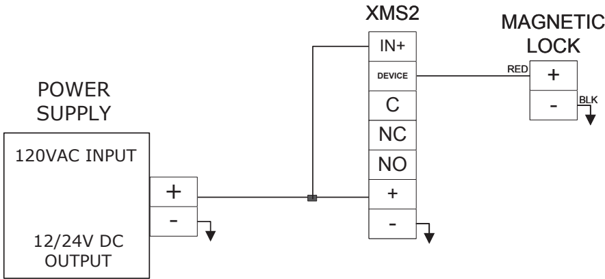
Diagram 10 Wiring Magnetic Lock Only
