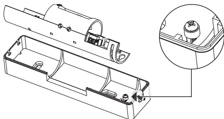
Diagram 6 Back Bracket
