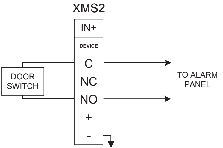
Diagram 12 Alarm Signal Closed with Door Closed
