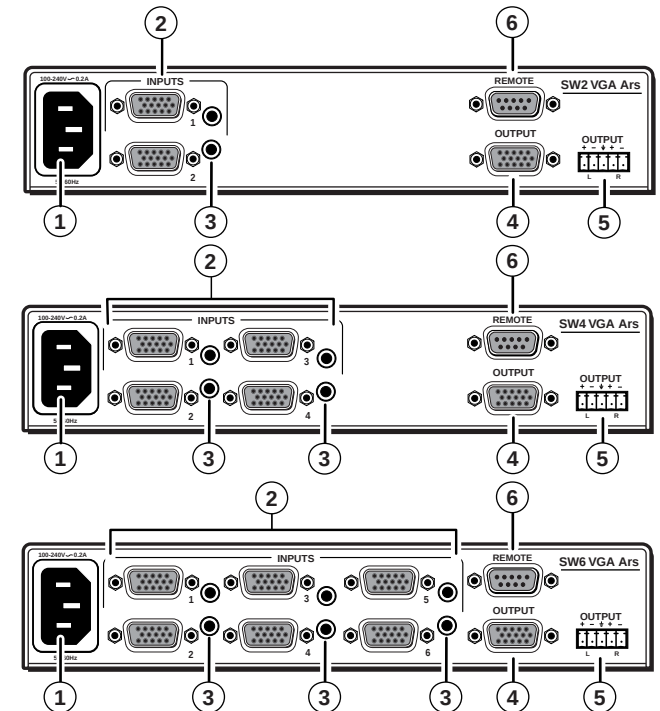
Figure 2-4 — Rear panel - SW VGA Ars switchers (with audio input and output connectors)
