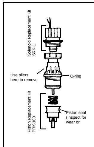
Actuator AVA-100-P
