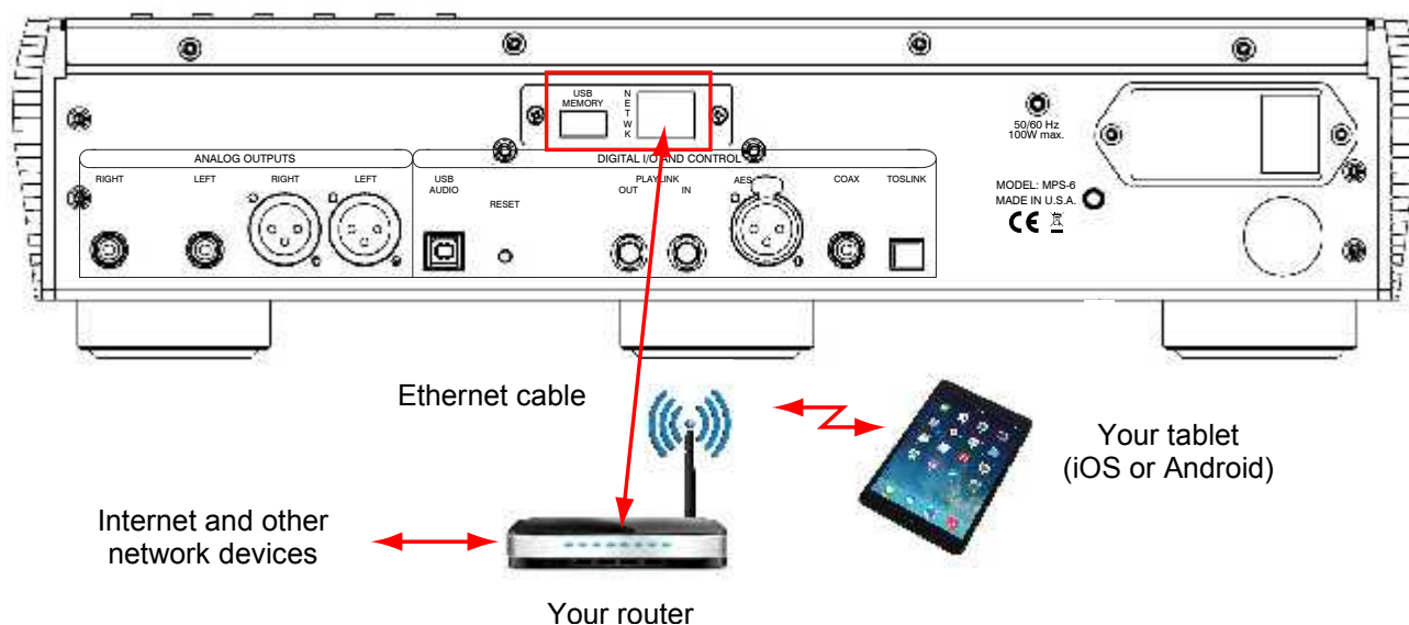
Stream-X2 connections on back panel of MPS-6
