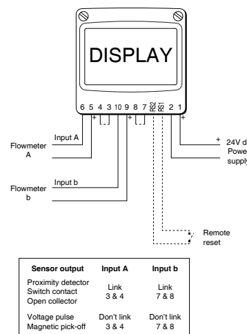
Fig 3 Typical measurement loop
