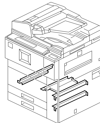
69. LOWER FRAME 1
