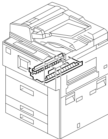
40. TRANSFER BELT UNIT 2
