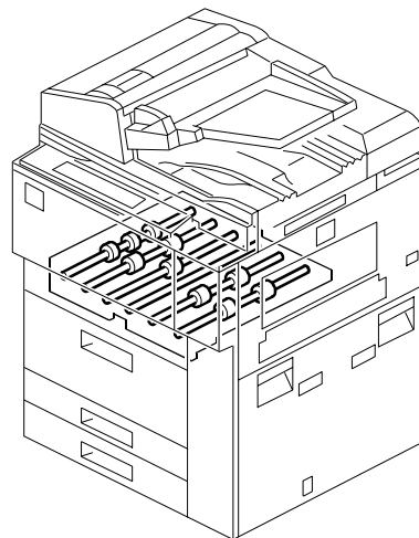
53. DUPLEX UNIT 4
