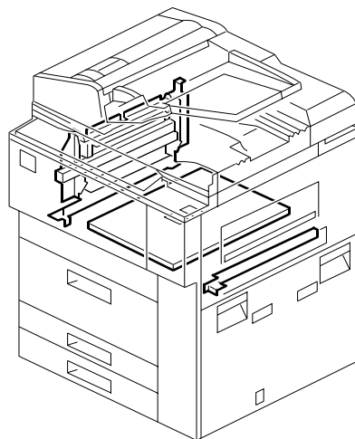
68. UPPER FRAME 3
