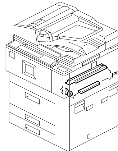
33. DEVELOPMENT UNIT 1
