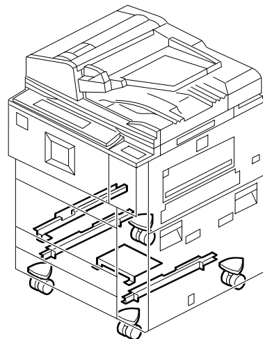
70. LOWER FRAME 2
