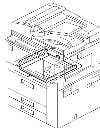
54. DUPLEX UNIT 5
