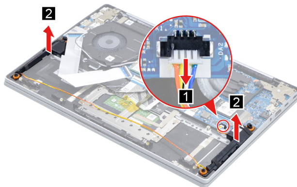
Figure 17. Remove the speakers
