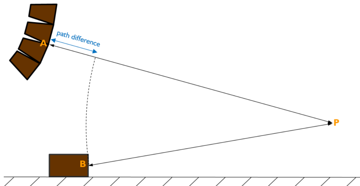
Illustrated example 1: line source + separated subwoofer
