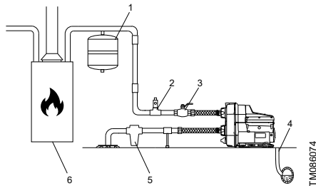
Installation example
