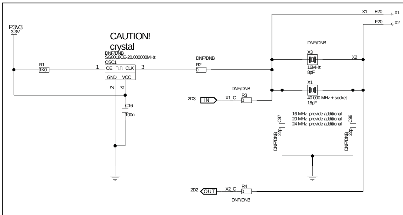
Figure 4.1 Clock supply
