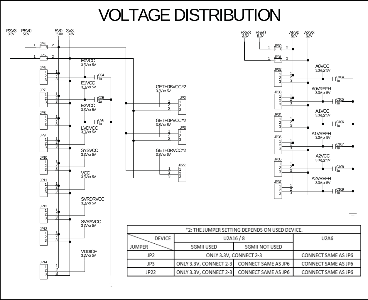
Figure 3.1 Voltage distribution
