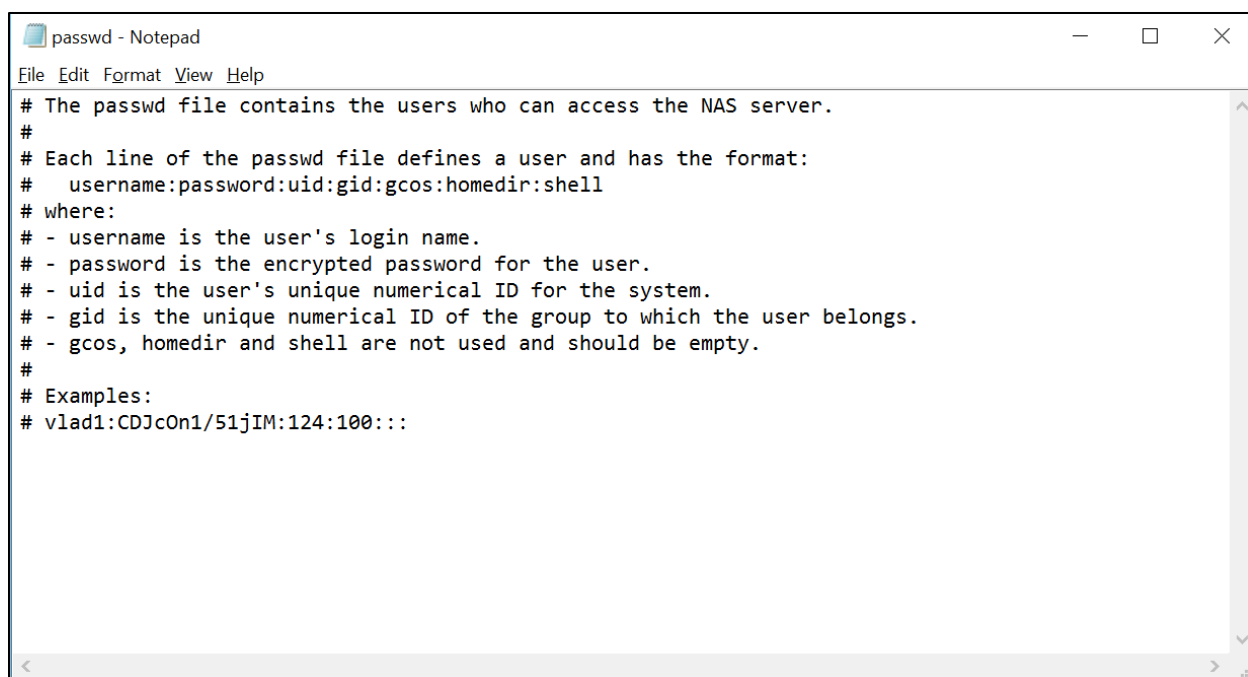
Figure 27 Passwd file
