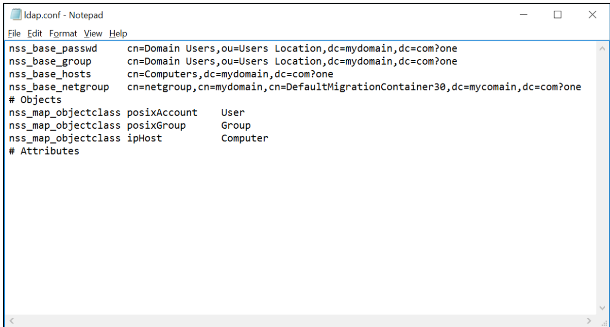
Figure 26 LDAP.conf
