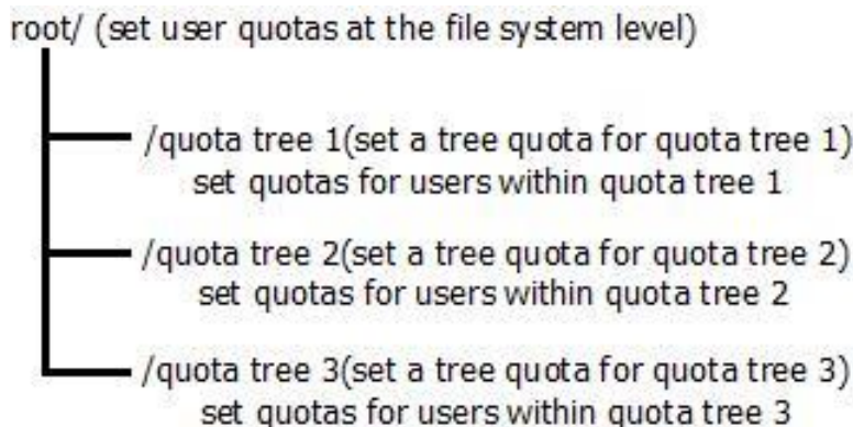
Figure 20 Quota hierarchy
