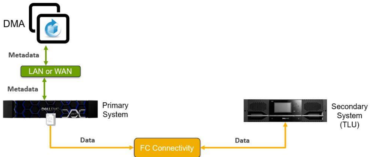
Figure 38 2-Way NDMP
