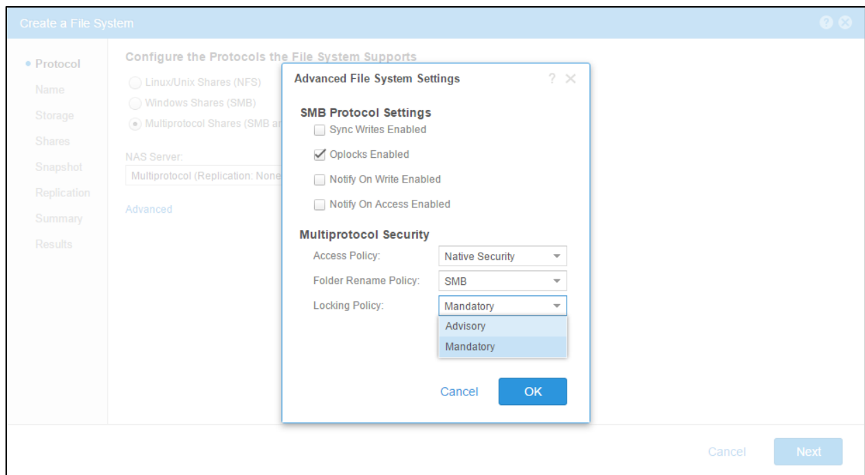
Figure 35 Locking policy
