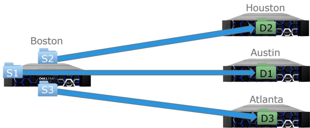
Figure 40 Replication
