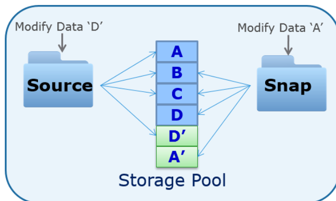
Figure 37 Unified snapshots
