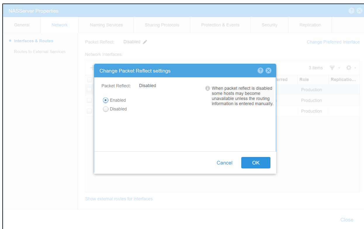
Figure 4 Packet reflect
