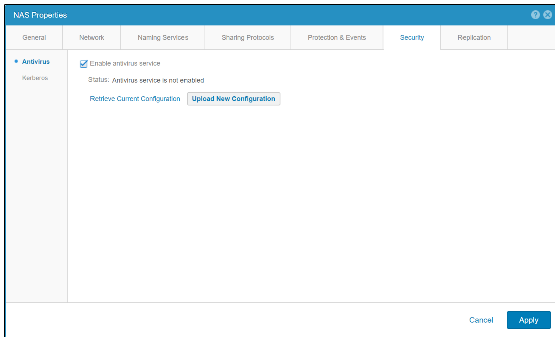
Figure 46 CEE CAVA
