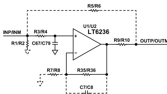
Figure 6. Stage 1 Simplified Schematic
