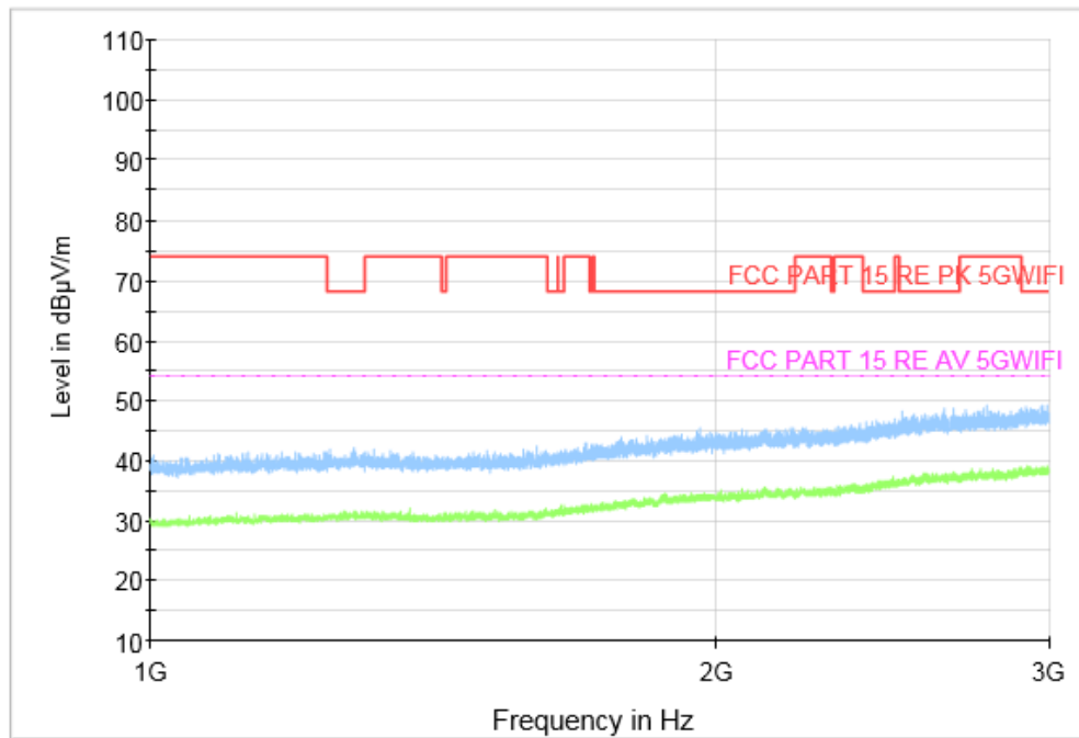
Fig. 39 Transmitter Spurious Emission (802. 11a, CH157 5785MHz, 1 GHz-3 GHz), SISO
