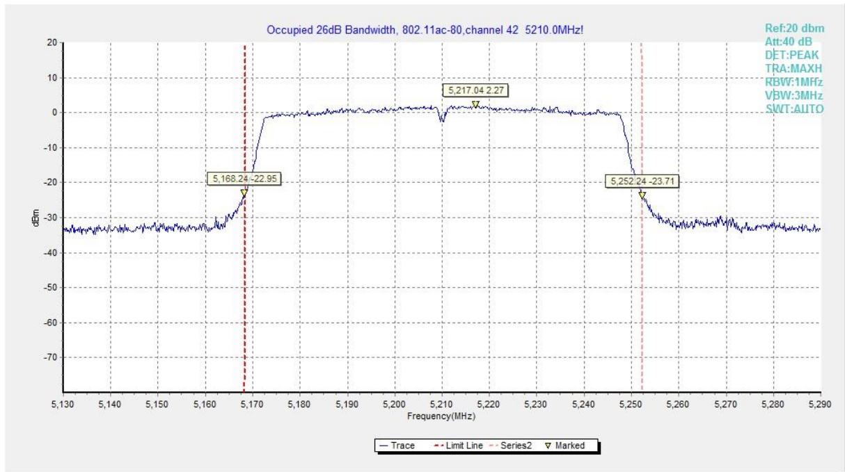
Fig. 6 Occupied 26dB Bandwidth (802. 11ac-VHT80, 5210MHz)
