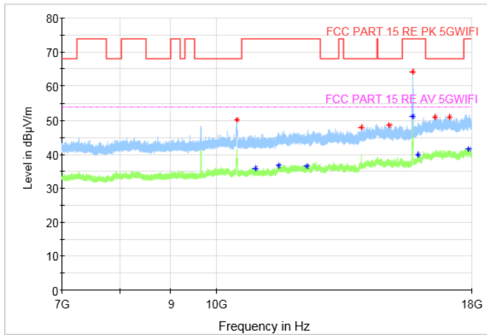
Fig. 35 Transmitter Spurious Emission (802.11a, CH48 5240MHz, 7 GHz-18 GHz), SISO
