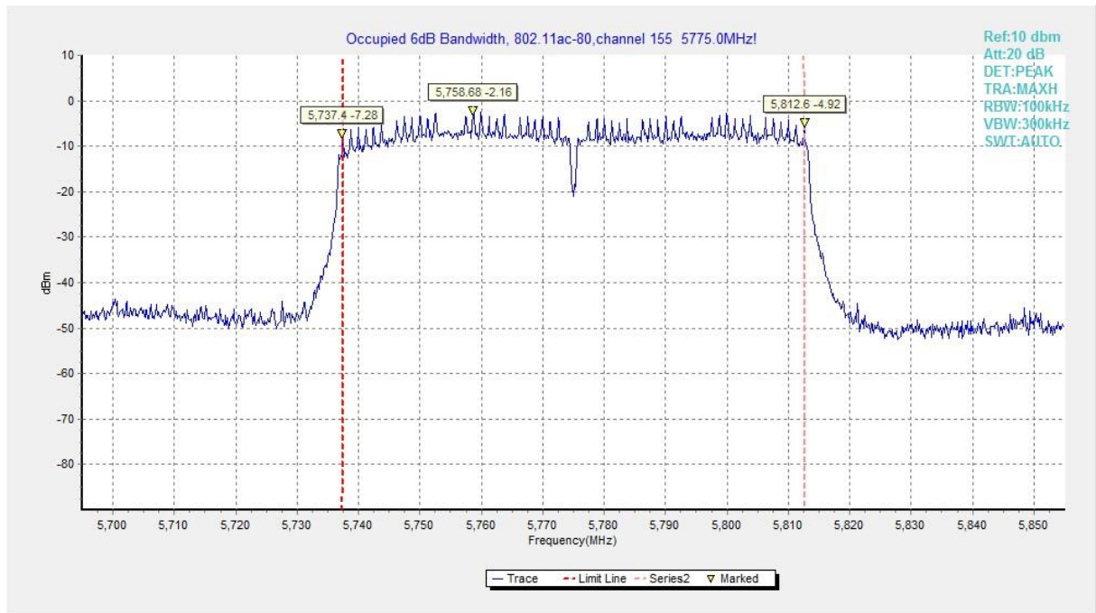
Fig. 12 Occupied 6dB Bandwidth (802.11ac-VHT80, 5775MHz)
