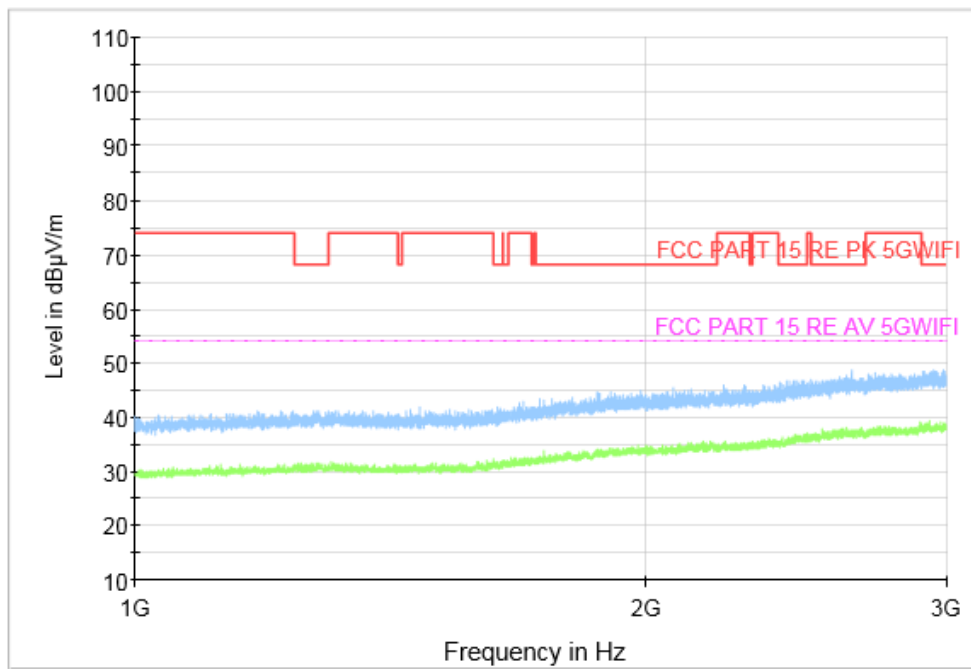
Fig. 45 Transmitter Spurious Emission (802.11n-HT40, CH38 5190MHz, 1 GHz-3 GHz), SISO
