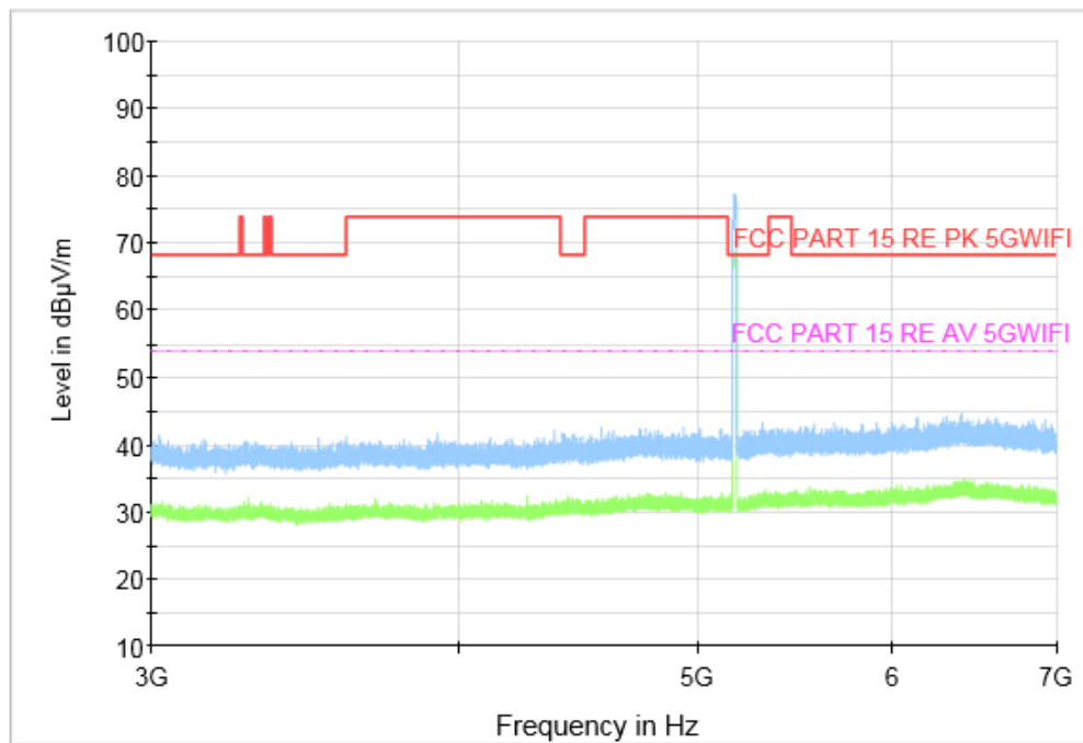
Fig. 28 Transmitter Spurious Emission (802.11a, CH36 5180MHz, 3 GHz-7 GHz), SISO
