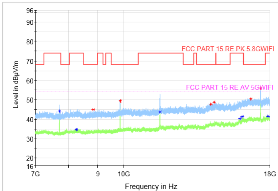
Fig. 41 Transmitter Spurious Emission (802. 11a, CH157 5785MHz, 7 GHz-18 GHz), SISO
