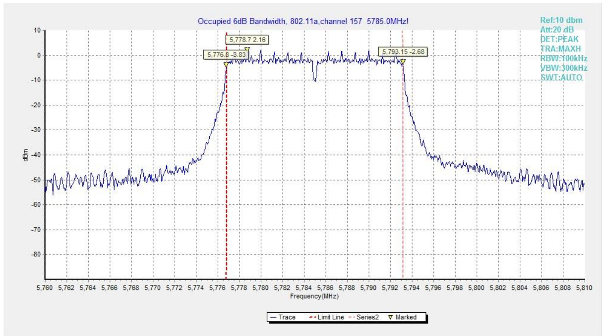
Fig. 8 Occupied 6dB Bandwidth (802.11a, 5785MHz)
