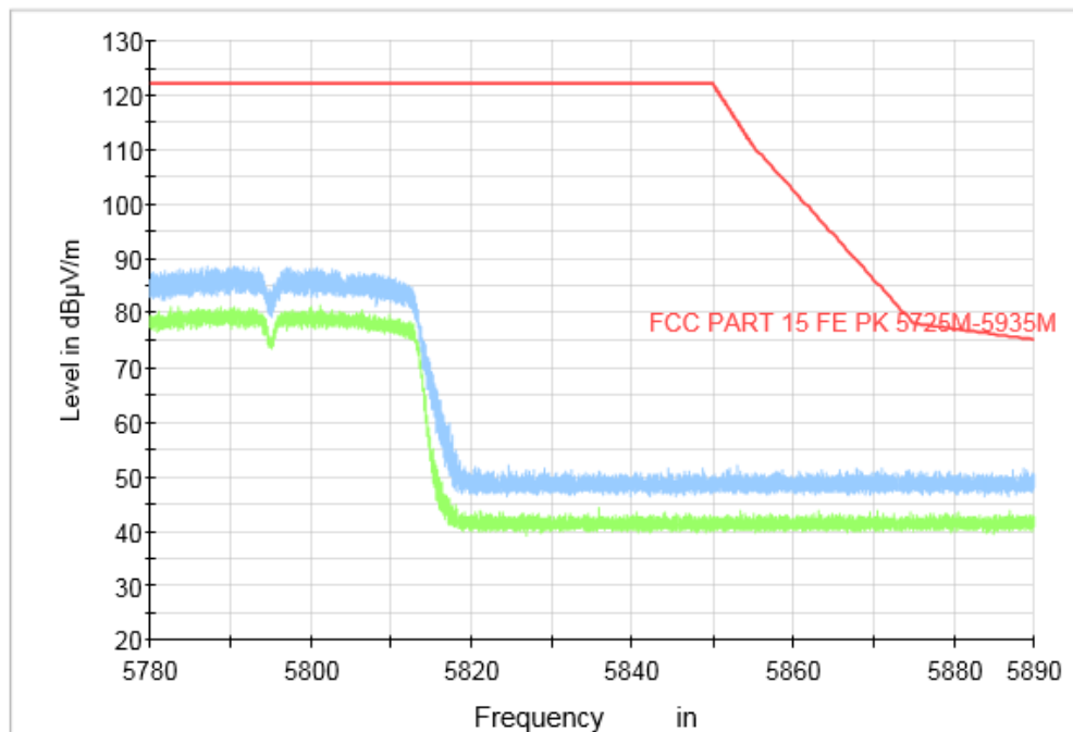
Fig. 24 Band Edges (802.11n-HT40, CH159 5795MHz)
