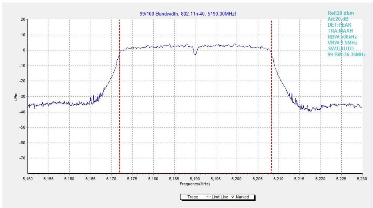
Fig. 16 99% Occupied Bandwidth (802.11n-HT40, 5190MHz)
