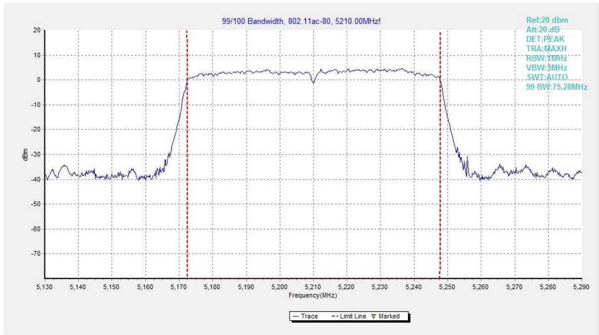
Fig. 18 99% Occupied Bandwidth (802.11ac-VHT80, 5210MHz)
