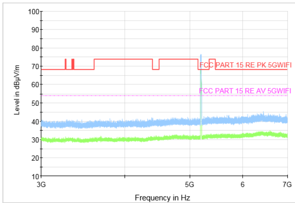
Fig. 31 Transmitter Spurious Emission (802.11a, CH40 5200MHz, 3 GHz-7 GHz), SISO
