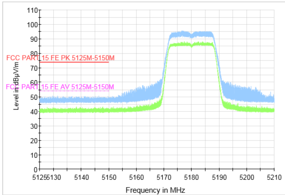
Fig. 19 Band Edges (802.11a, CH36 5180MHz)
