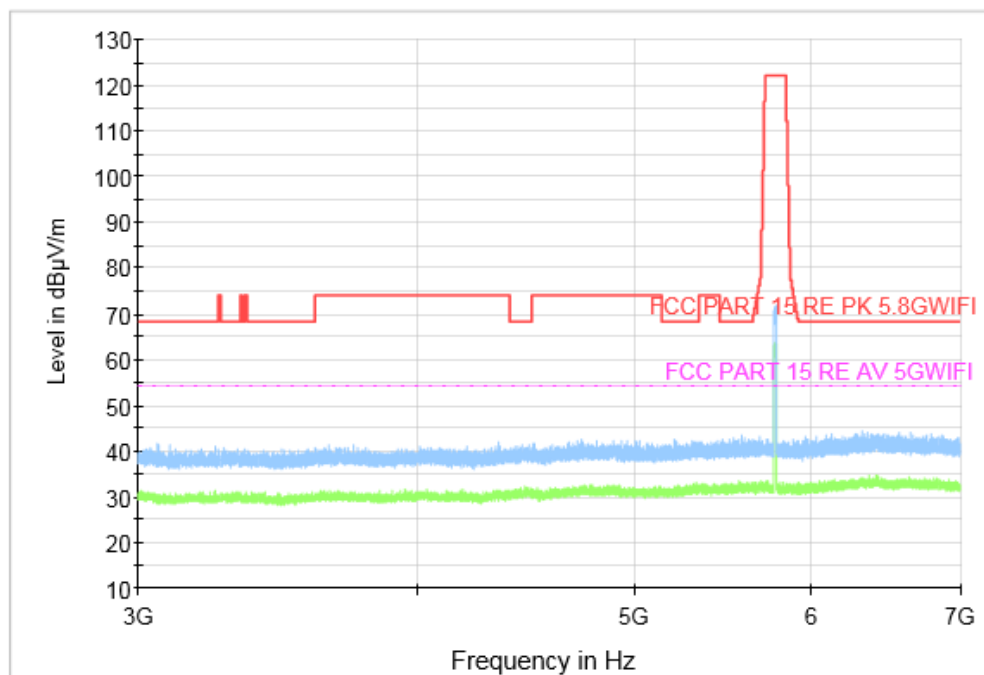
Fig. 40 Transmitter Spurious Emission (802. 11a, CH157 5785MHz, 3 GHz-7 GHz), SISO
