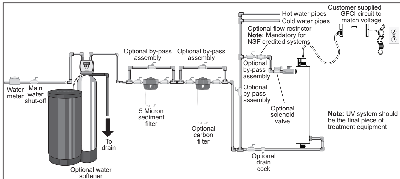
Figure 3 Disinfection System
