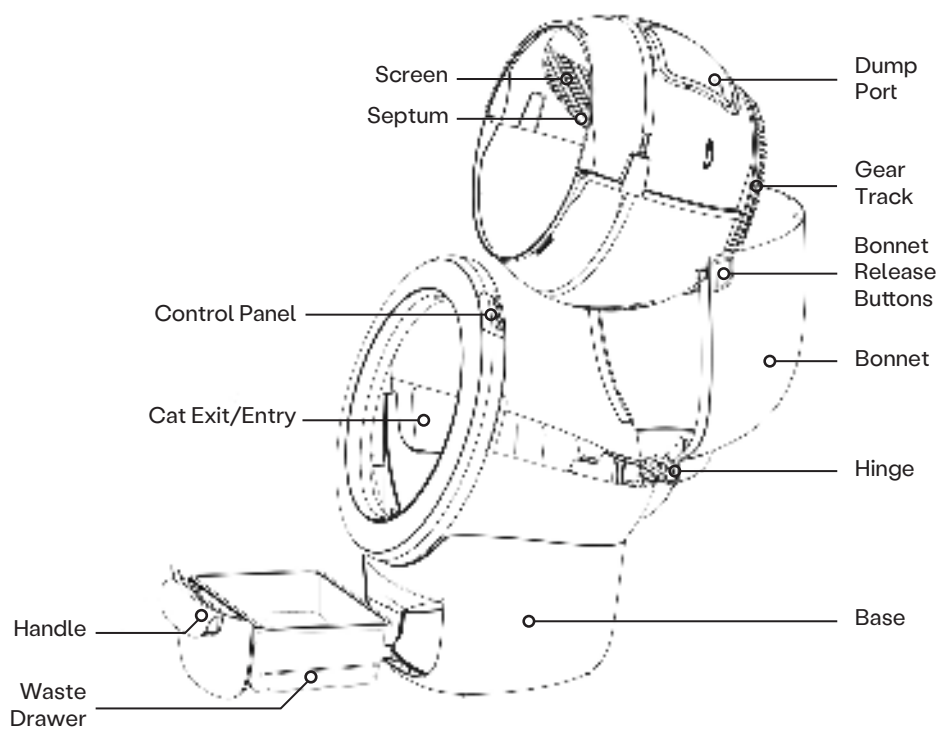
Exploded View
