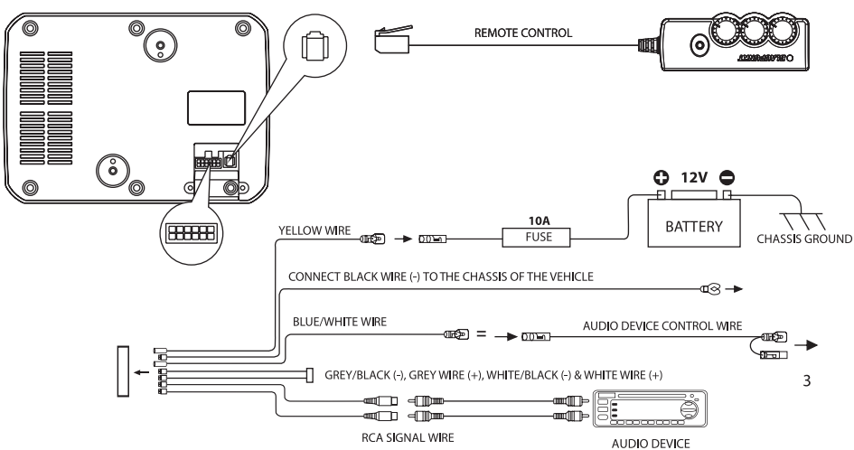
Diagram 2 (Low Level Input -RCA Input)
